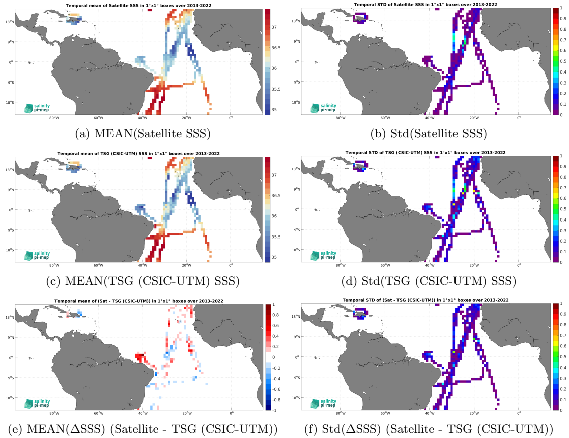
Figure 7: Temporal mean (left) and Std (right) of SSS from SMAP SSS L4 OI v3 - Monthly (ESR) (top), TSG (CSIC-UTM) (middle), and of \Delta\text{SSS} (Satellite - TSG (CSIC-UTM)). Only match-up pairs are used to generate these maps.
