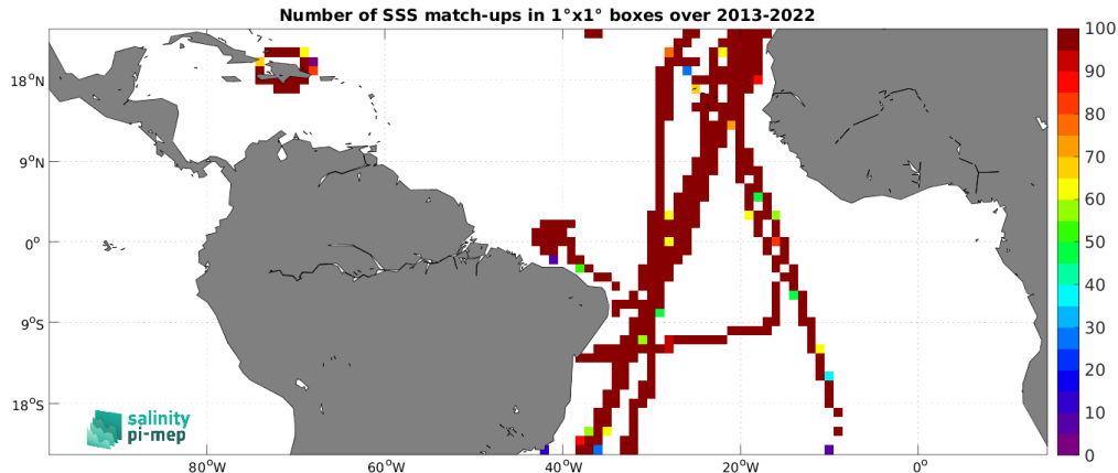
Figure 5: Number of SSS match-ups between TSG (CSIC-UTM) SSS and the SMAP SSS L4 OI v3 - Monthly (ESR) SSS product for the Tropical Atlantic Ocean Pi-MEP region over 1^\circ \times 1^\circ boxes and for the full satellite product period.
