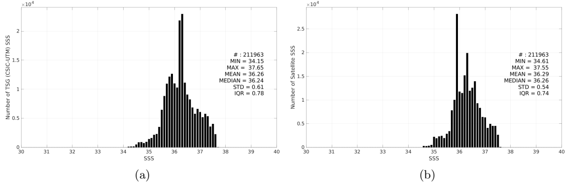
Figure 3: Histograms of SSS from TSG (CSIC-UTM) (a) and SMAP SSS L4 OI v3 - Monthly (ESR) (b) considering all match-up pairs per bins of 0.1 over the Tropical Atlantic Ocean Pi-MEP region and for the full satellite product period.
