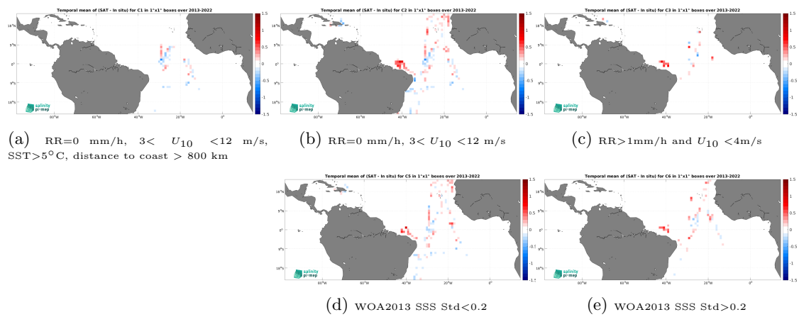
Figure 14: Temporal mean gridded over spatial boxes of size 1^\circ \times 1^\circ of \Delta\text{SSS} (SMAP SSS L4 OI v3 - Monthly (ESR) - TSG (CSIC-UTM)) for 5 different subdatasets corresponding to:RR=0 mm/h, 3 < U_{10} < 12 m/s, SST >5^\circ\text{C} , distance to coast > 800 km (a), RR=0 mm/h, 3 < U_{10} < 12 m/s (b), RR >1 mm/h and U_{10} < 4 m/s (c), WOA2013 SSS Std <0.2 (d), WOA2013 SSS Std >0.2 (e).
