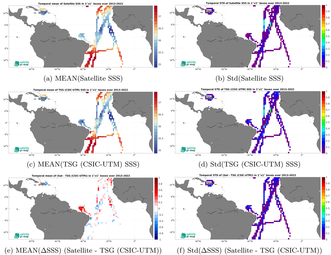
Figure 7: Temporal mean (left) and Std (right) of SSS from SMAP SSS L4 OI v3 - Monthly (ESR) (top), TSG (CSIC-UTM) (middle), and of \Delta SSS (Satellite - TSG (CSIC-UTM)). Only match-up pairs are used to generate these maps.
