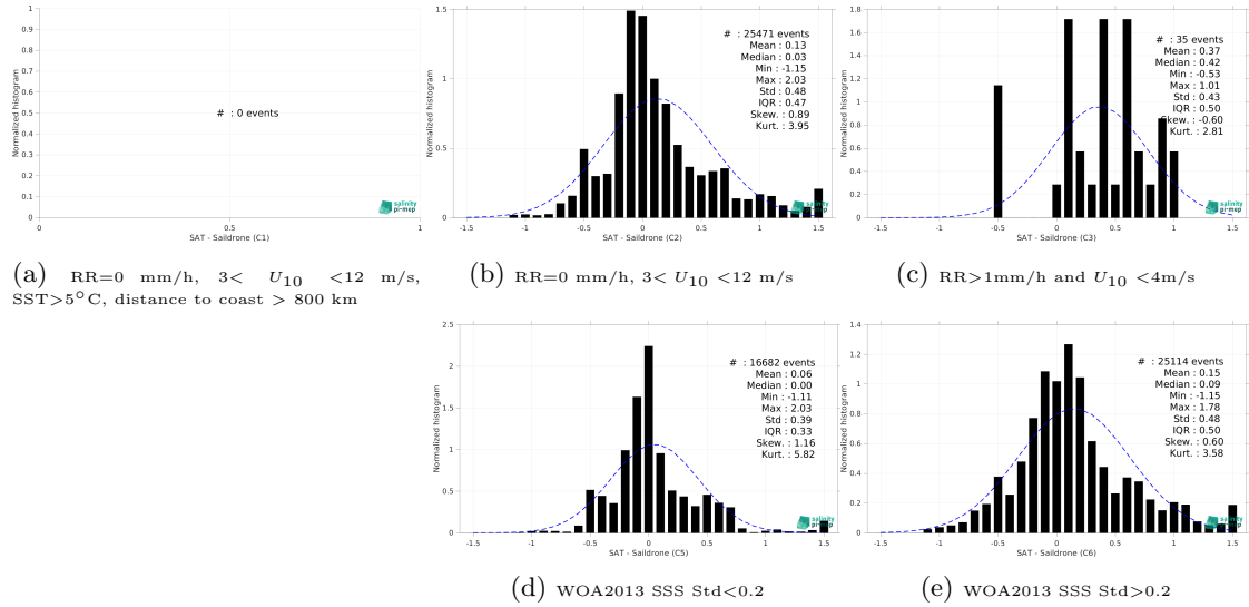
Figure 15: Normalized histogram of \Delta SSS (SMAP SSS L4 OI v3 - Monthly (ESR) - Sairdron) for 5 different subdatasets corresponding to: RR=0 mm/h, 3 < U_{10} < 12 m/s, SST > 5°C, distance to coast > 800 km (a), RR=0 mm/h, 3 < U_{10} < 12 m/s (b), RR > 1mm/h and U_{10} < 4 m/s (c), WOA2013 SSS Std < 0.2 (d), WOA2013 SSS Std > 0.2 (e).
