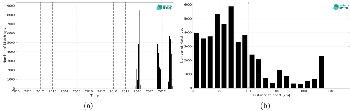
Figure 2: Number of match-ups between Saildrone and SMAP SSS L4 OI v3 - Monthly (ESR) SSS as a function of time (a) and as function of the distance to coast (b) over the Tropical Atlantic Ocean Pi-MEP region and for the full satellite product period.
