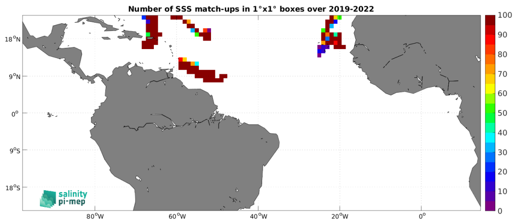
Figure 5: Number of SSS match-ups between Saildrone SSS and the SMAP SSS L4 OI v3 - Monthly (ESR) SSS product for the Tropical Atlantic Ocean Pi-MEP region over 1^\circ \times 1^\circ boxes and for the full satellite product period.
