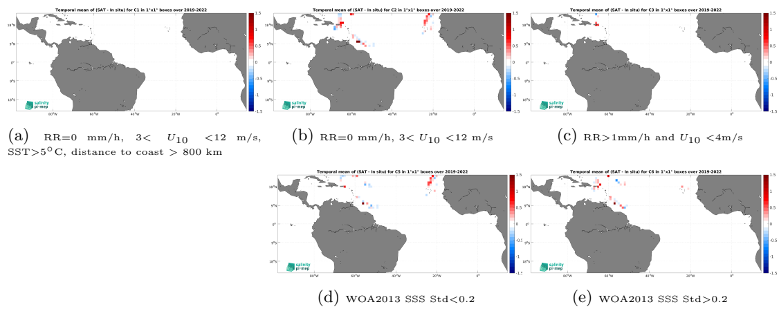
Figure 14: Temporal mean gridded over spatial boxes of size 1^\circ \times 1^\circ of \Delta SSS (SMAP SSS L4 OI v3 - Monthly (ESR) - Sairdrone) for 5 different subdatasets corresponding to:RR=0 mm/h, 3 < U_{10} < 12 m/s, SST >5^\circ\text{C} , distance to coast > 800 km (a), RR=0 mm/h, 3 < U_{10} < 12 m/s (b), RR >1 mm/h and U_{10} < 4 m/s (c), WOA2013 SSS Std <0.2 (d), WOA2013 SSS Std >0.2 (e).
