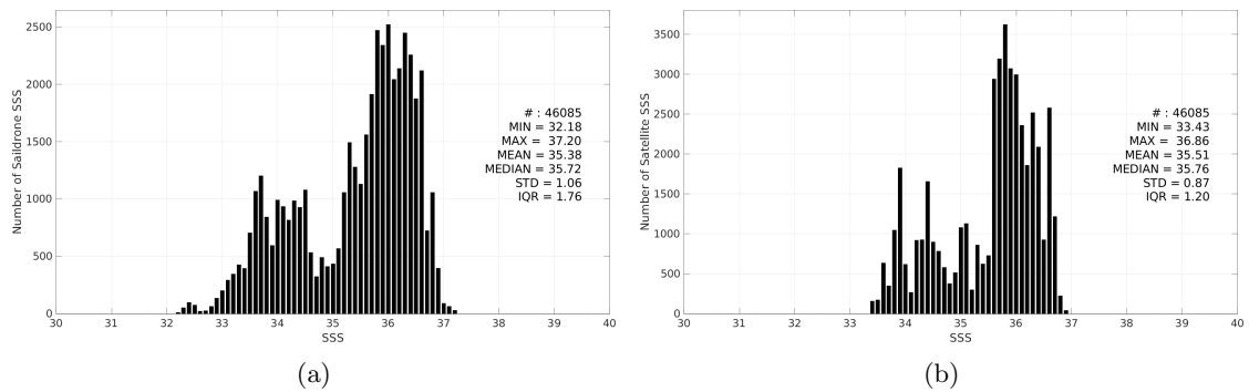
Figure 3: Histograms of SSS from Saildrone (a) and SMAP SSS L4 OI v3 - Monthly (ESR) (b) considering all match-up pairs per bins of 0.1 over the Tropical Atlantic Ocean Pi-MEP region and for the full satellite product period.
