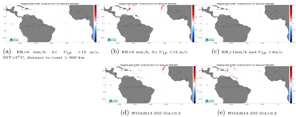
Figure 14: Temporal mean gridded over spatial boxes of size 1^\circ \times 1^\circ of \Delta\text{SSS} (SMAP SSS L4 OI v3 - Monthly (ESR) - Saildrone) for 5 different subdatasets corresponding to:RR=0 mm/h, 3 < U_{10} < 12 m/s, SST>5°C, distance to coast > 800 km (a), RR=0 mm/h, 3 < U_{10} < 12 m/s (b), RR>1mm/h and U_{10} < 4 m/s (c), WOA2013 SSS Std<0.2 (d), WOA2013 SSS Std>0.2 (e).
