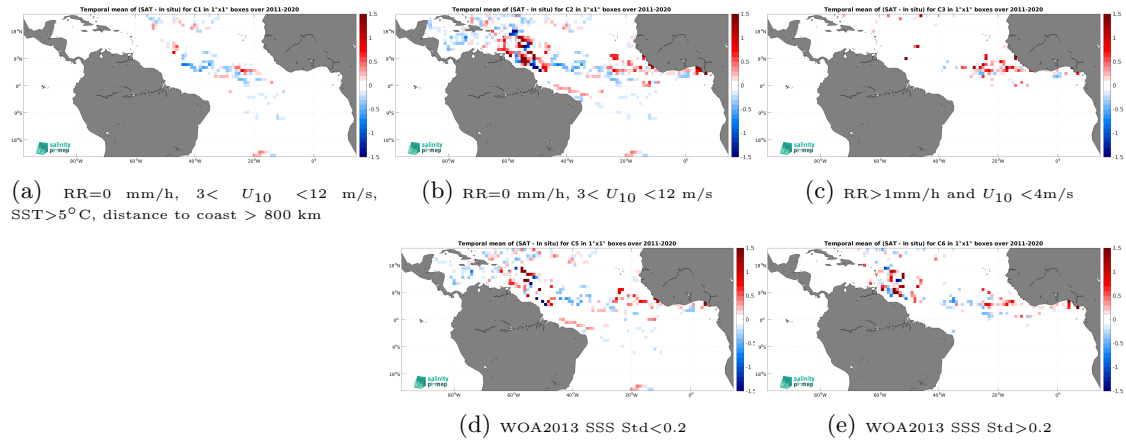
Figure 13: Temporal mean gridded over spatial boxes of size 1^\circ \times 1^\circ of \Delta SSS (SMAP SSS L4 OI v3 - Monthly (ESR) - Surface drifters) for 5 different subdatasets corresponding to:RR=0 mm/h, 3 < U_{10} < 12 m/s, SST >5^\circ\text{C} , distance to coast > 800 km (a), RR=0 mm/h, 3 < U_{10} < 12 m/s (b), RR >1 mm/h and U_{10} < 4 m/s (c), WOA2013 SSS Std <0.2 (d), WOA2013 SSS Std >0.2 (e).
