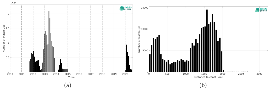
Figure 2: Number of match-ups between Surface drifters and SMAP SSS L4 OI v3 - Monthly (ESR) SSS as a function of time (a) and as function of the distance to coast (b) over the Tropical Atlantic Ocean Pi-MEP region and for the full satellite product period.
