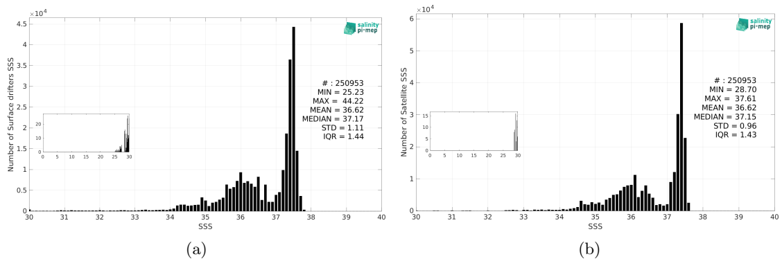
Figure 3: Histograms of SSS from Surface drifters (a) and SMAP SSS L4 OI v3 - Monthly (ESR) (b) considering all match-up pairs per bins of 0.1 over the Tropical Atlantic Ocean Pi-MEP region and for the full satellite product period.
