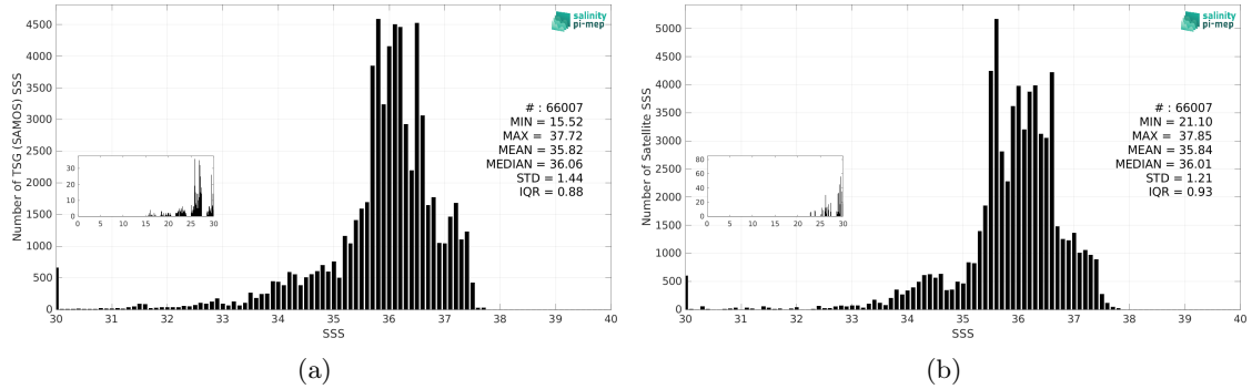
Figure 3: Histograms of SSS from TSG (SAMOS) (a) and SMAP SSS L4 OI v3 - Daily (ESR) (b) considering all match-up pairs per bins of 0.1 over the Tropical Atlantic Ocean Pi-MEP region and for the full satellite product period.
