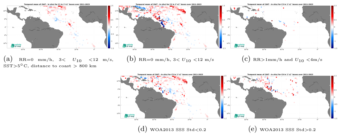
Figure 14: Temporal mean gridded over spatial boxes of size 1^\circ \times 1^\circ of \Delta\text{SSS} (SMAP SSS L4 OI v3 - Daily (ESR) - TSG (SAMOS)) for 5 different subdatasets corresponding to:RR=0 mm/h, 3 < U_{10} < 12 m/s, SST >5^\circ\text{C} , distance to coast > 800 km (a), RR=0 mm/h, 3 < U_{10} < 12 m/s (b), RR >1 mm/h and U_{10} < 4 m/s (c), WOA2013 SSS Std <0.2 (d), WOA2013 SSS Std >0.2 (e).
