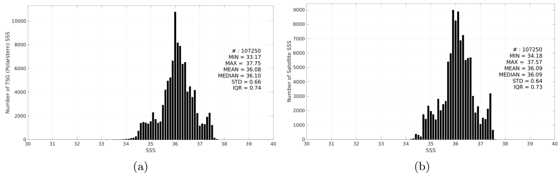
Figure 3: Histograms of SSS from TSG (Polarstern) (a) and SMAP SSS L4 OI v3 - Daily (ESR) (b) considering all match-up pairs per bins of 0.1 over the Tropical Atlantic Ocean Pi-MEP region and for the full satellite product period.
