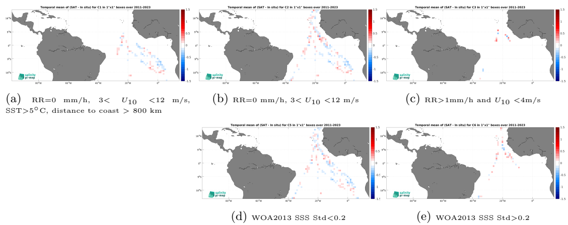
Figure 14: Temporal mean gridded over spatial boxes of size 1^\circ \times 1^\circ of \Delta\text{SSS} (SMAP SSS L4 OI v3 - Daily (ESR) - TSG (Polarstern)) for 5 different subdatasets corresponding to:RR=0 mm/h, 3 < U_{10} < 12 m/s, SST >5^\circ\text{C} , distance to coast > 800 km (a), RR=0 mm/h, 3 < U_{10} < 12 m/s (b), RR >1 mm/h and U_{10} < 4 m/s (c), WOA2013 SSS Std <0.2 (d), WOA2013 SSS Std >0.2 (e).
