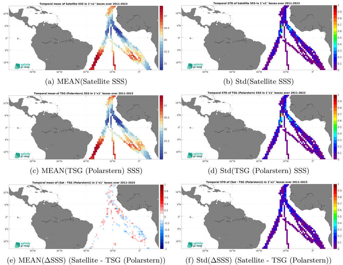
Figure 7: Temporal mean (left) and Std (right) of SSS from SMAP SSS L4 OI v3 - Daily (ESR) (top), TSG (Polarstern) (middle), and of \Delta SSS (Satellite - TSG (Polarstern)). Only match-up pairs are used to generate these maps.
