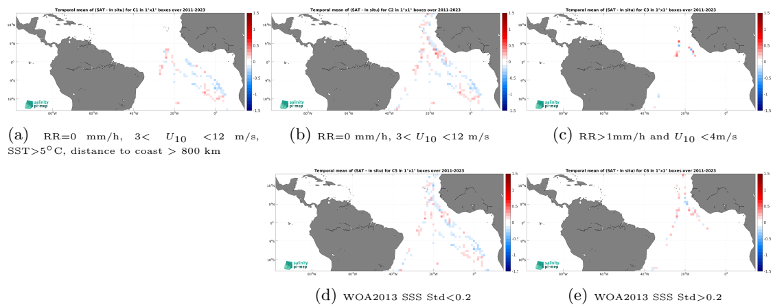
Figure 14: Temporal mean gridded over spatial boxes of size 1^\circ \times 1^\circ of \Delta\text{SSS} (SMAP SSS L4 OI v3 - Daily (ESR) - TSG (Polarstern)) for 5 different subdatasets corresponding to:RR=0 mm/h, 3 < U_{10} < 12 m/s, SST >5^\circ\text{C} , distance to coast > 800 km (a), RR=0 mm/h, 3 < U_{10} < 12 m/s (b), RR >1 mm/h and U_{10} < 4 m/s (c), WOA2013 SSS Std <0.2 (d), WOA2013 SSS Std >0.2 (e).
