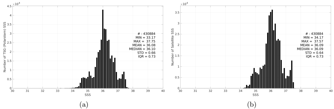
Figure 3: Histograms of SSS from TSG (Polarstern) (a) and SMAP SSS L4 OI v3 - Daily (ESR) (b) considering all match-up pairs per bins of 0.1 over the Tropical Atlantic Ocean Pi-MEP region and for the full satellite product period.
