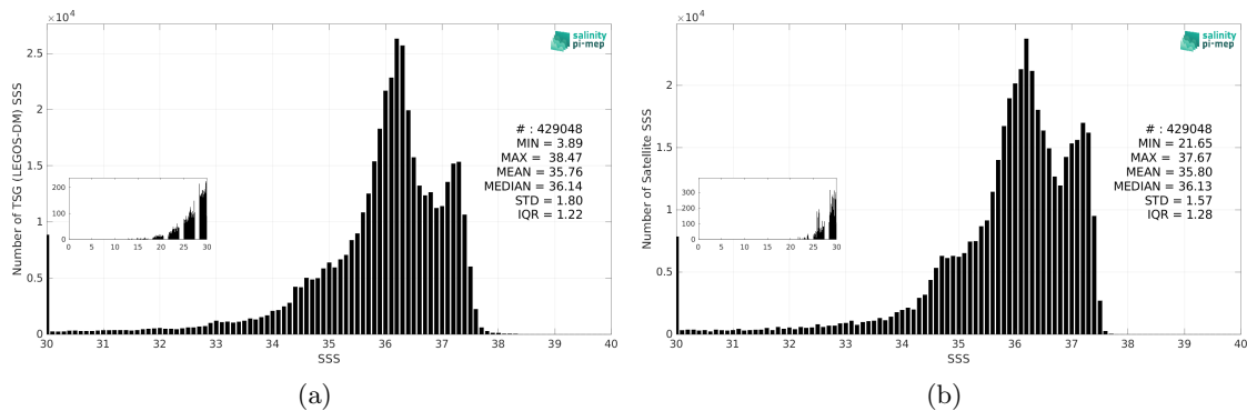
Figure 3: Histograms of SSS from TSG (LEGOS-DM) (a) and SMAP SSS L4 OI v3 - Daily (ESR) (b) considering all match-up pairs per bins of 0.1 over the Tropical Atlantic Ocean Pi-MEP region and for the full satellite product period.
