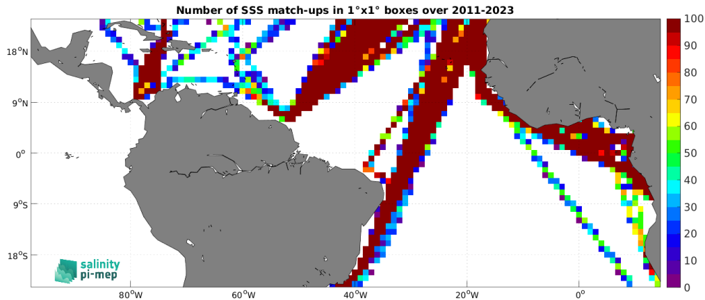
Figure 5: Number of SSS match-ups between TSG (LEGOS-DM) SSS and the SMAP SSS L4 OI v3 - Daily (ESR) SSS product for the Tropical Atlantic Ocean Pi-MEP region over 1^\circ \times 1^\circ boxes and for the full satellite product period.
