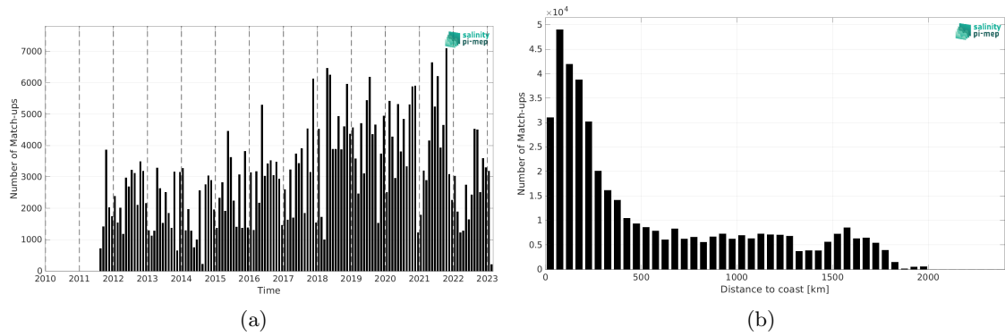
Figure 2: Number of match-ups between TSG (LEGOS-DM) and SMAP SSS L4 OI v3 - Daily (ESR) SSS as a function of time (a) and as function of the distance to coast (b) over the Tropical Atlantic Ocean Pi-MEP region and for the full satellite product period.
