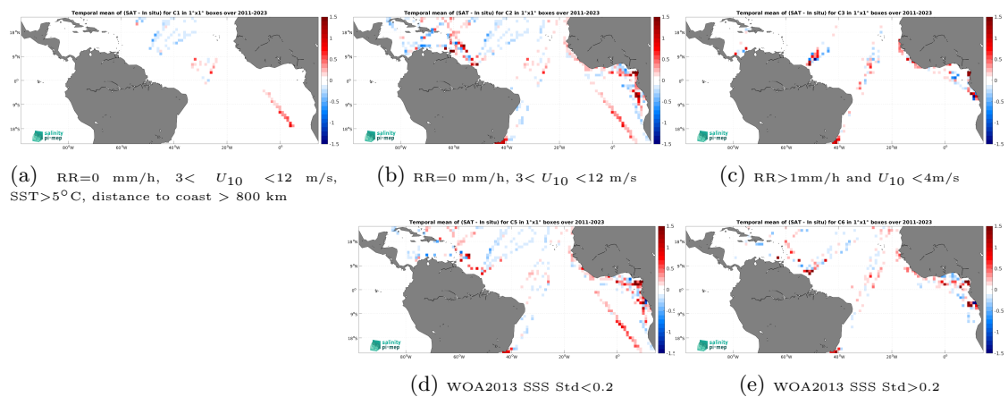
Figure 14: Temporal mean gridded over spatial boxes of size 1^\circ \times 1^\circ of \Delta\text{SSS} (SMAP SSS L4 OI v3 - Daily (ESR) - TSG (LEGOS-DM)) for 5 different subdatasets corresponding to:RR=0 mm/h, 3 < U_{10} < 12 m/s, SST >5^\circ\text{C} , distance to coast > 800 km (a), RR=0 mm/h, 3 < U_{10} < 12 m/s (b), RR >1 mm/h and U_{10} < 4 m/s (c), WOA2013 SSS Std <0.2 (d), WOA2013 SSS Std >0.2 (e).
