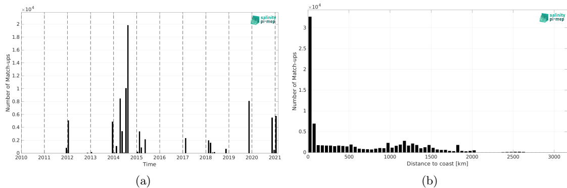
Figure 2: Number of match-ups between TSG (GOSUD-Sailing-ship) and SMAP SSS L4 OI v3 - Daily (ESR) SSS as a function of time (a) and as function of the distance to coast (b) over the Tropical Atlantic Ocean Pi-MEP region and for the full satellite product period.
