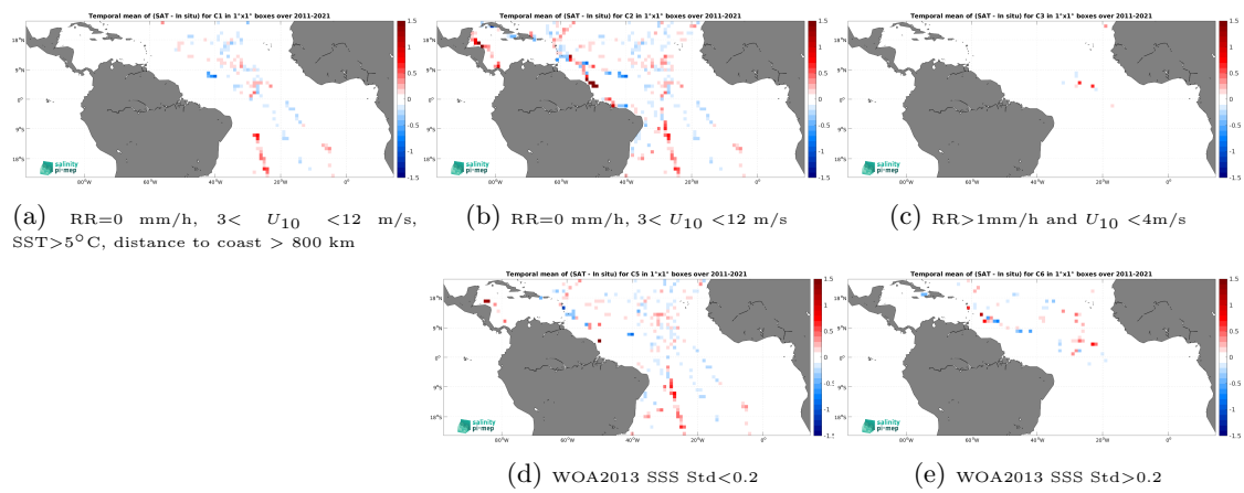
Figure 14: Temporal mean gridded over spatial boxes of size 1^\circ \times 1^\circ of \Delta\text{SSS} (SMAP SSS L4 OI v3 - Daily (ESR) - TSG (GOSUD-Sailing-ship)) for 5 different subdatasets corresponding to:RR=0 mm/h, 3 < U_{10} < 12 m/s, SST >5^\circ\text{C} , distance to coast > 800 km (a), RR=0 mm/h, 3 < U_{10} < 12 m/s (b), RR >1 mm/h and U_{10} < 4 m/s (c), WOA2013 SSS Std <0.2 (d), WOA2013 SSS Std >0.2 (e).
