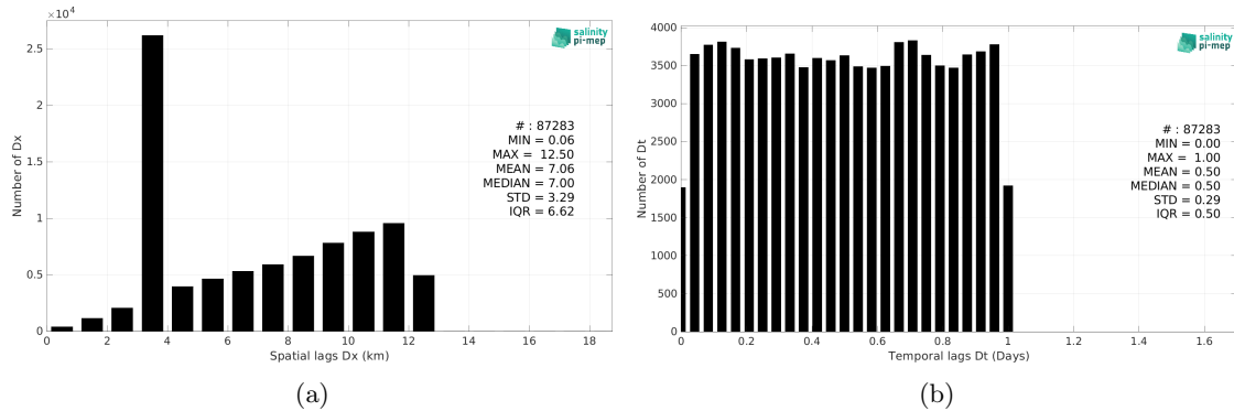
Figure 6: Histograms of the spatial (a) and temporal (b) lags between the location/time of the TSG (GOSUD-Sailing-ship) measurement and the date of the corresponding SMAP SSS L4 OI v3 - Daily (ESR) SSS pixel.
