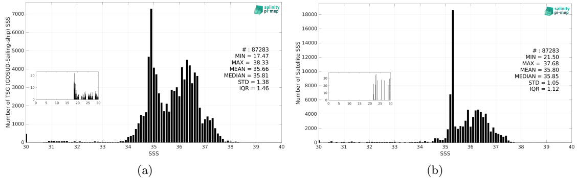
Figure 3: Histograms of SSS from TSG (GOSUD-Sailing-ship) (a) and SMAP SSS L4 OI v3 - Daily (ESR) (b) considering all match-up pairs per bins of 0.1 over the Tropical Atlantic Ocean Pi-MEP region and for the full satellite product period.
