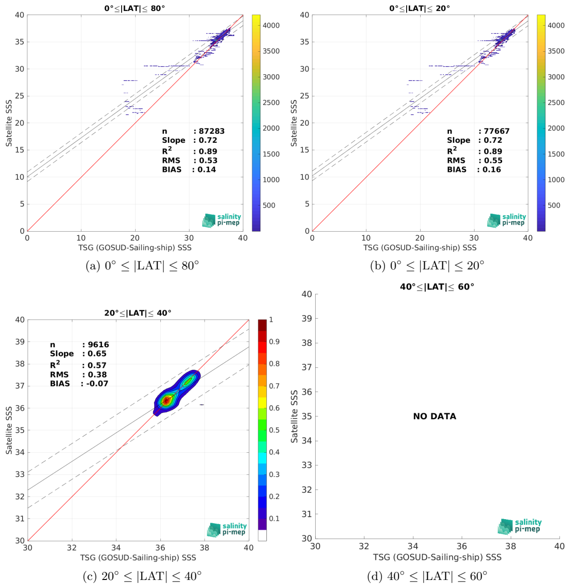
Figure 10: Contour maps of the concentration of SMAP SSS L4 OI v3 - Daily (ESR) SSS (y-axis) versus TSG (GOSUD-Sailing-ship) SSS (x-axis) at match-up pairs for different latitude bands. For each plot, the red line shows x=y . The black thin and dashed lines indicate a linear fit through the data cloud and the \pm 95\% confidence levels, respectively. The number match-up pairs n , the slope and R^2 coefficient of the linear fit, the root mean square (RMS) and the mean bias between satellite and in situ data are indicated for each latitude band in each plots.
