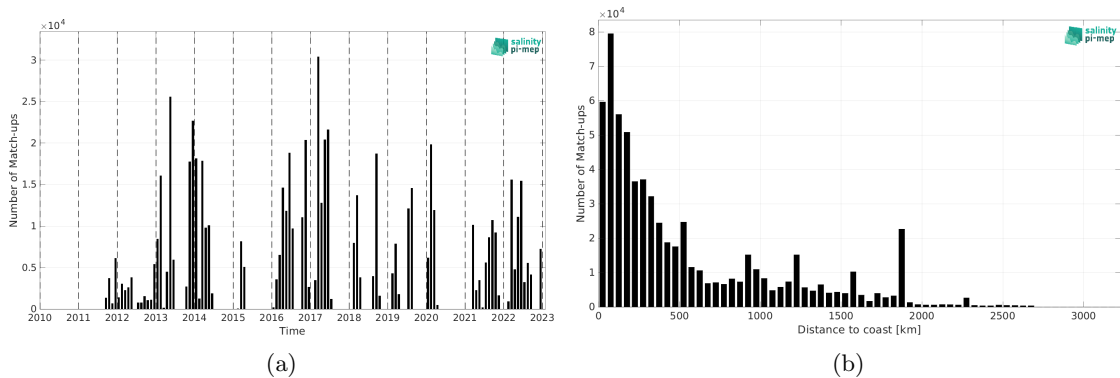
Figure 2: Number of match-ups between TSG (GOSUD-Research-vessel) and SMAP SSS L4 OI v3 - Daily (ESR) SSS as a function of time (a) and as function of the distance to coast (b) over the Tropical Atlantic Ocean Pi-MEP region and for the full satellite product period.
