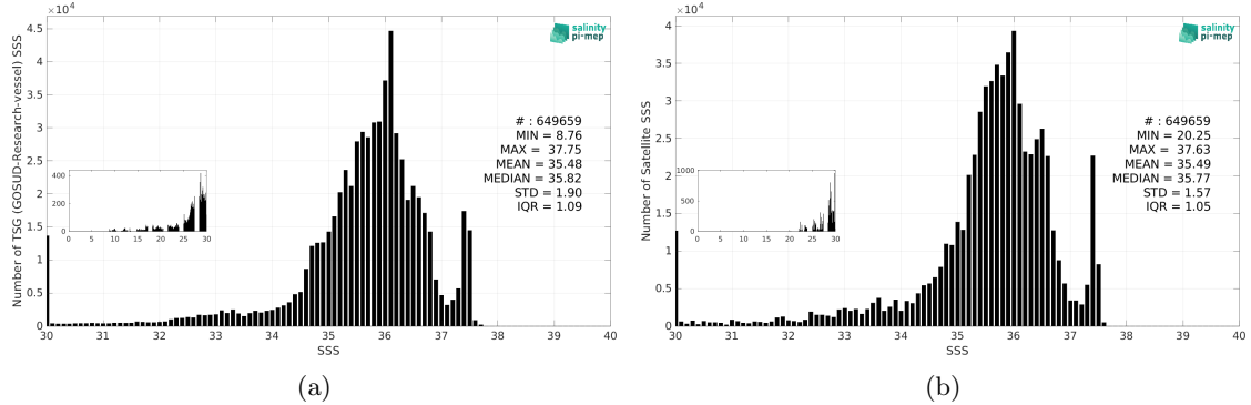
Figure 3: Histograms of SSS from TSG (GOSUD-Research-vessel) (a) and SMAP SSS L4 OI v3 - Daily (ESR) (b) considering all match-up pairs per bins of 0.1 over the Tropical Atlantic Ocean Pi-MEP region and for the full satellite product period.
