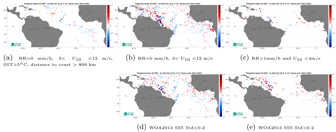
Figure 14: Temporal mean gridded over spatial boxes of size 1^\circ \times 1^\circ of \Delta\text{SSS} (SMAP SSS L4 OI v3 - Daily (ESR) - TSG (GOSUD-Research-vessel)) for 5 different subdatasets corresponding to:RR=0 mm/h, 3 < U_{10} < 12 m/s, SST >5^\circ\text{C} , distance to coast > 800 km (a), RR=0 mm/h, 3 < U_{10} < 12 m/s (b), RR >1 mm/h and U_{10} < 4 m/s (c), WOA2013 SSS Std <0.2 (d), WOA2013 SSS Std >0.2 (e).
