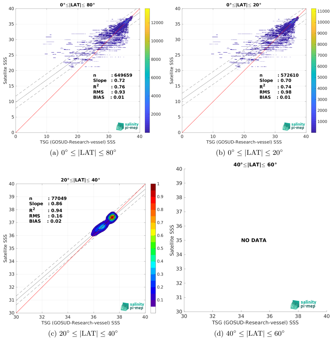
Figure 10: Contour maps of the concentration of SMAP SSS L4 OI v3 - Daily (ESR) SSS (y-axis) versus TSG (GOSUD-Research-vessel) SSS (x-axis) at match-up pairs for different latitude bands. For each plot, the red line shows x=y . The black thin and dashed lines indicate a linear fit through the data cloud and the \pm 95\% confidence levels, respectively. The number match-up pairs n , the slope and R^2 coefficient of the linear fit, the root mean square (RMS) and the mean bias between satellite and in situ data are indicated for each latitude band in each plots.
