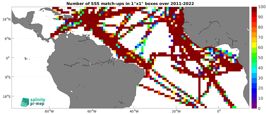
Figure 5: Number of SSS match-ups between TSG (GOSUD-Research-vessel) SSS and the SMAP SSS L4 OI v3 - Daily (ESR) SSS product for the Tropical Atlantic Ocean Pi-MEP region over 1^\circ \times 1^\circ boxes and for the full satellite product period.
