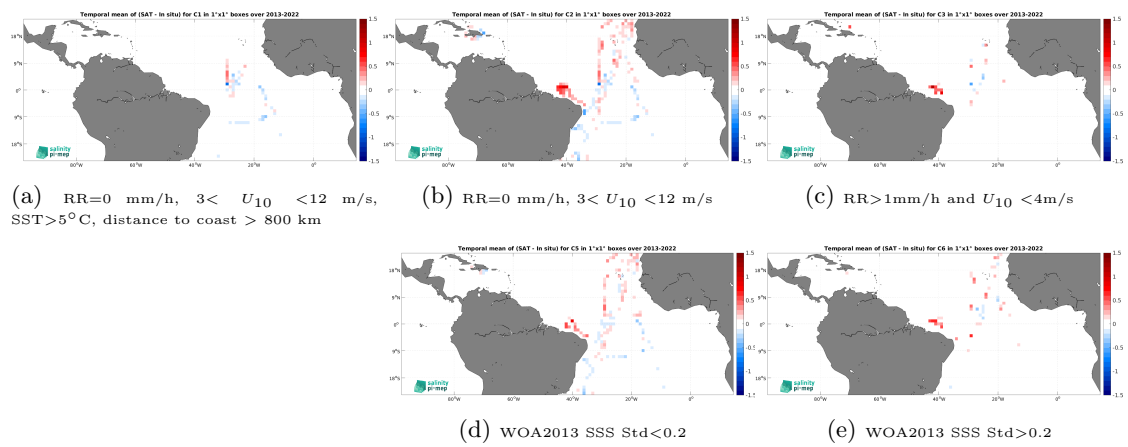
Figure 14: Temporal mean gridded over spatial boxes of size 1^\circ \times 1^\circ of \Delta\text{SSS} (SMAP SSS L4 OI v3 - Daily (ESR) - TSG (CSIC-UTM)) for 5 different subdatasets corresponding to:RR=0 mm/h, 3 < U_{10} < 12 m/s, SST >5^\circ\text{C} , distance to coast > 800 km (a), RR=0 mm/h, 3 < U_{10} < 12 m/s (b), RR >1 mm/h and U_{10} < 4 m/s (c), WOA2013 SSS Std <0.2 (d), WOA2013 SSS Std >0.2 (e).
