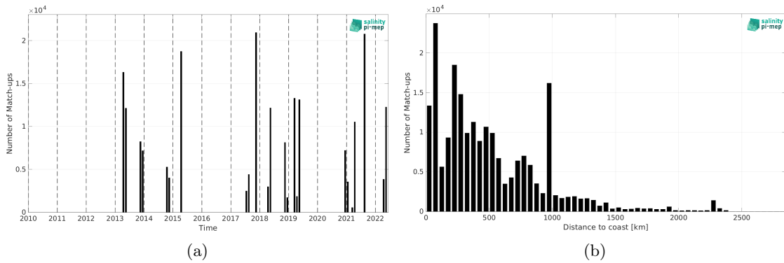
Figure 2: Number of match-ups between TSG (CSIC-UTM) and SMAP SSS L4 OI v3 - Daily (ESR) SSS as a function of time (a) and as function of the distance to coast (b) over the Tropical Atlantic Ocean Pi-MEP region and for the full satellite product period.
