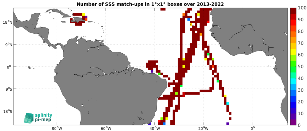
Figure 5: Number of SSS match-ups between TSG (CSIC-UTM) SSS and the SMAP SSS L4 OI v3 - Daily (ESR) SSS product for the Tropical Atlantic Ocean Pi-MEP region over 1^\circ \times 1^\circ boxes and for the full satellite product period.
