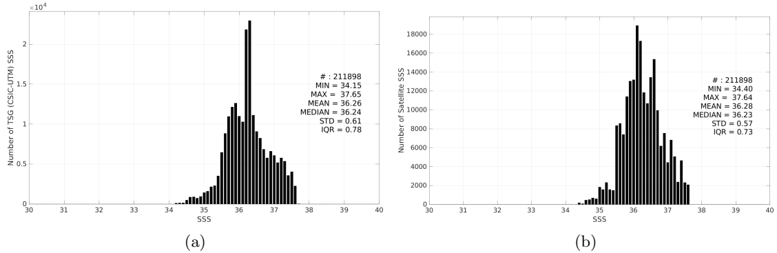
Figure 3: Histograms of SSS from TSG (CSIC-UTM) (a) and SMAP SSS L4 OI v3 - Daily (ESR) (b) considering all match-up pairs per bins of 0.1 over the Tropical Atlantic Ocean Pi-MEP region and for the full satellite product period.
