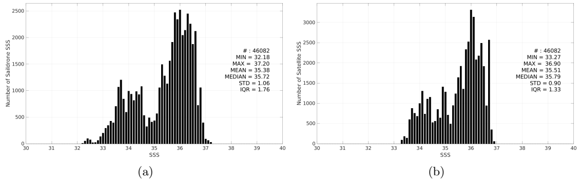
Figure 3: Histograms of SSS from Saildrone (a) and SMAP SSS L4 OI v3 - Daily (ESR) (b) considering all match-up pairs per bins of 0.1 over the Tropical Atlantic Ocean Pi-MEP region and for the full satellite product period.
