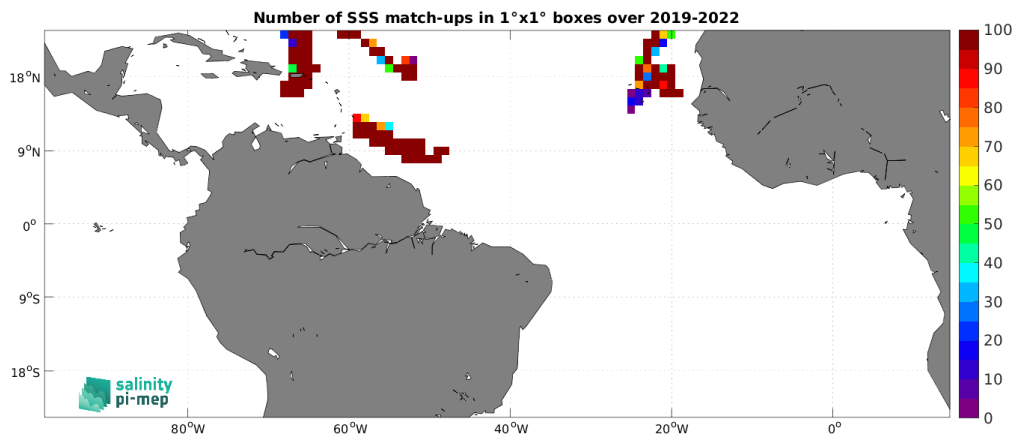
Figure 5: Number of SSS match-ups between Saildrone SSS and the SMAP SSS L4 OI v3 - Daily (ESR) SSS product for the Tropical Atlantic Ocean Pi-MEP region over 1^\circ \times 1^\circ boxes and for the full satellite product period.
