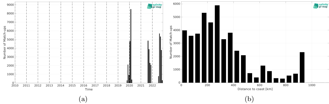
Figure 2: Number of match-ups between Saildrone and SMAP SSS L4 OI v3 - Daily (ESR) SSS as a function of time (a) and as function of the distance to coast (b) over the Tropical Atlantic Ocean Pi-MEP region and for the full satellite product period.
