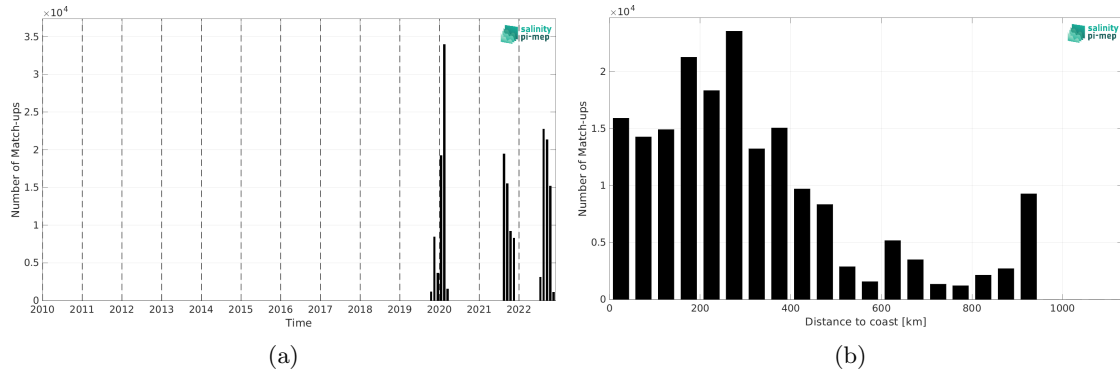
Figure 2: Number of match-ups between Saildrone and SMAP SSS L4 OI v3 - Daily (ESR) SSS as a function of time (a) and as function of the distance to coast (b) over the Tropical Atlantic Ocean Pi-MEP region and for the full satellite product period.
