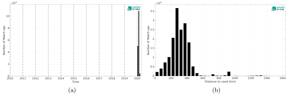
Figure 2: Number of match-ups between EUREC4A and SMAP SSS L4 OI v3 - Daily (ESR) SSS as a function of time (a) and as function of the distance to coast (b) over the Tropical Atlantic Ocean Pi-MEP region and for the full satellite product period.
