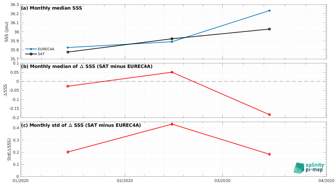
Figure 8: Time series of the monthly median SSS (top), median of \Delta SSS (Satellite - EUREC4A) and Std of \Delta SSS (Satellite - EUREC4A) over the Tropical Atlantic Ocean Pi-MEP region considering all match-ups collected by the Pi-MEP.
