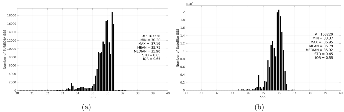
Figure 3: Histograms of SSS from EUREC4A (a) and SMAP SSS L4 OI v3 - Daily (ESR) (b) considering all match-up pairs per bins of 0.1 over the Tropical Atlantic Ocean Pi-MEP region and for the full satellite product period.
