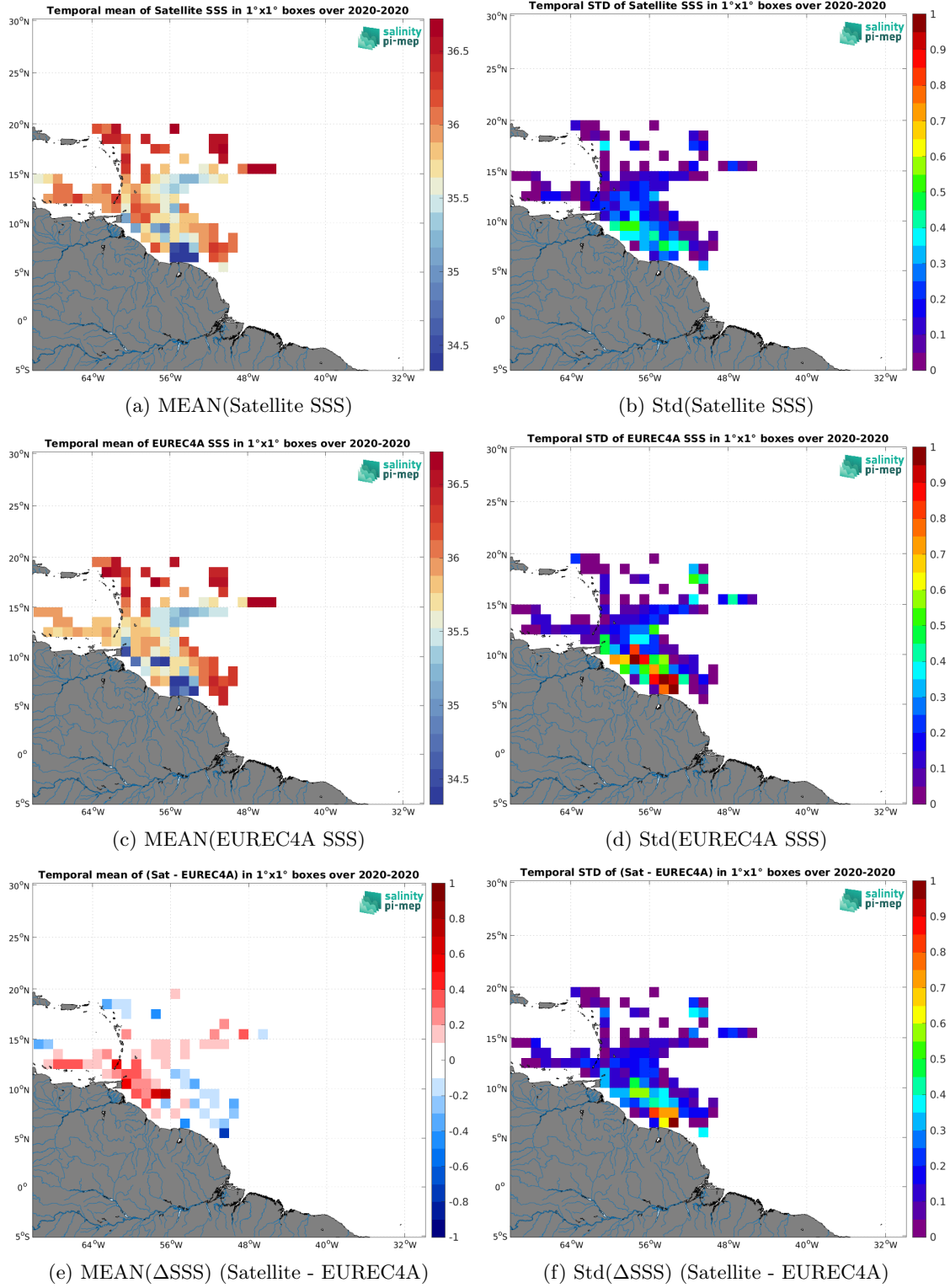
Figure 7: Temporal mean (left) and Std (right) of SSS from SMAP SSS L4 OI v3 - Daily (ESR) (top), EUREC4A (middle), and of \Delta SSS (Satellite - EUREC4A). Only match-up pairs are used to generate these maps.
