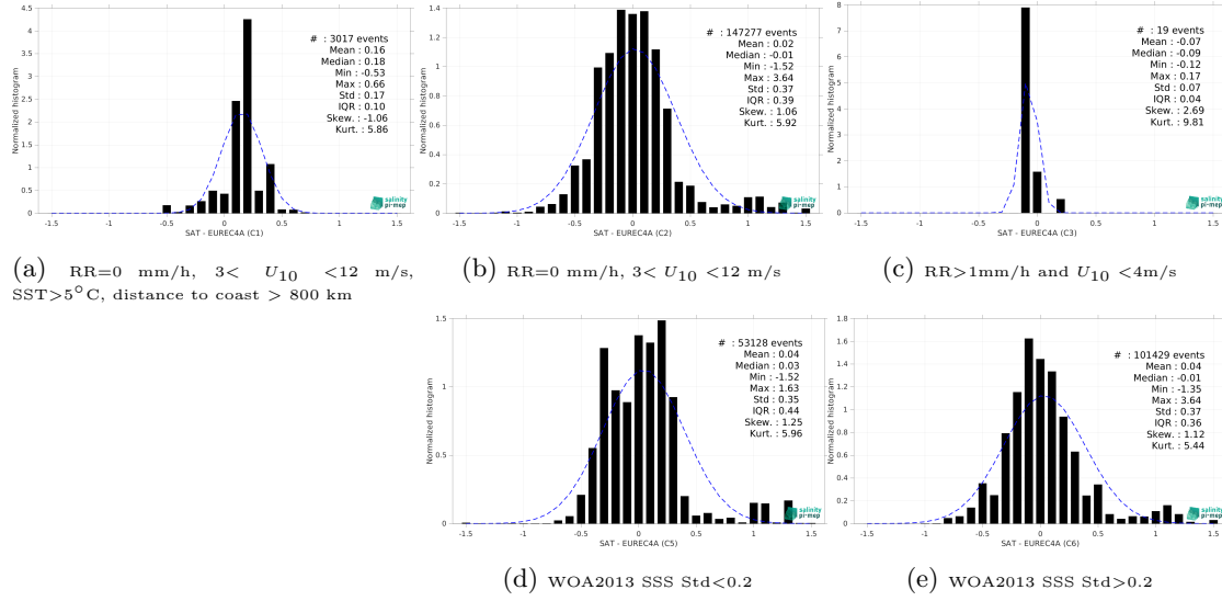
Figure 15: Normalized histogram of \Delta SSS (SMAP SSS L4 OI v3 - Daily (ESR) - EUREC4A) for 5 different subdatasets corresponding to: RR=0 mm/h, 3 < U_{10} < 12 m/s, SST>5°C, distance to coast > 800 km (a), RR=0 mm/h, 3 < U_{10} < 12 m/s (b), RR>1mm/h and U_{10} < 4 m/s (c), WOA2013 SSS Std<0.2 (d), WOA2013 SSS Std>0.2 (e).
