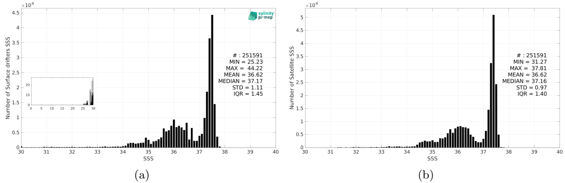
Figure 3: Histograms of SSS from Surface drifters (a) and SMAP SSS L4 OI v3 - Daily (ESR) (b) considering all match-up pairs per bins of 0.1 over the Tropical Atlantic Ocean Pi-MEP region and for the full satellite product period.
