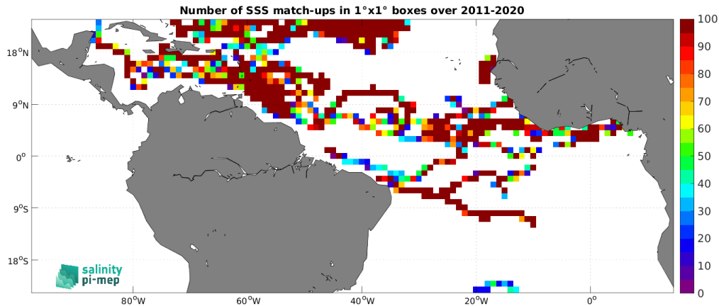
Figure 4: Number of SSS match-ups between Surface drifters SSS and the SMAP SSS L4 OI v3 - Daily (ESR) SSS product for the Tropical Atlantic Ocean Pi-MEP region over 1^\circ \times 1^\circ boxes and for the full satellite product period.
