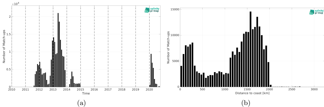
Figure 2: Number of match-ups between Surface drifters and SMAP SSS L4 OI v3 - Daily (ESR) SSS as a function of time (a) and as function of the distance to coast (b) over the Tropical Atlantic Ocean Pi-MEP region and for the full satellite product period.
