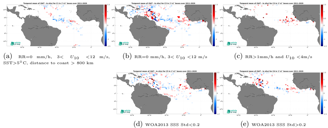
Figure 13: Temporal mean gridded over spatial boxes of size 1^\circ \times 1^\circ of \Delta\text{SSS} (SMAP SSS L4 OI v3 - Daily (ESR) - Surface drifters) for 5 different subdatasets corresponding to:RR=0 mm/h, 3 < U_{10} < 12 m/s, SST >5^\circ\text{C} , distance to coast > 800 km (a), RR=0 mm/h, 3 < U_{10} < 12 m/s (b), RR >1 mm/h and U_{10} < 4 m/s (c), WOA2013 SSS Std <0.2 (d), WOA2013 SSS Std >0.2 (e).
