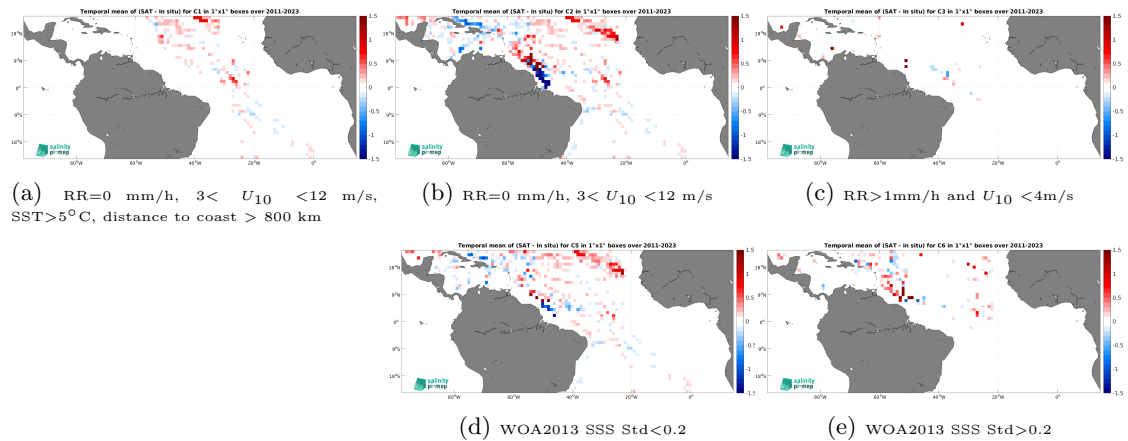
Figure 12: Temporal mean gridded over spatial boxes of size 1^\circ \times 1^\circ of \Delta\text{SSS} (SMAP SSS L4 OI v2 - 7 Days (ESR) - TSG (SAMOS)) for 5 different subdatasets corresponding to:RR=0 mm/h, 3 < U_{10} < 12 m/s, SST >5^\circ\text{C} , distance to coast > 800 km (a), RR=0 mm/h, 3 < U_{10} < 12 m/s (b), RR >1 mm/h and U_{10} < 4 m/s (c), WOA2013 SSS Std <0.2 (d), WOA2013 SSS Std >0.2 (e).
