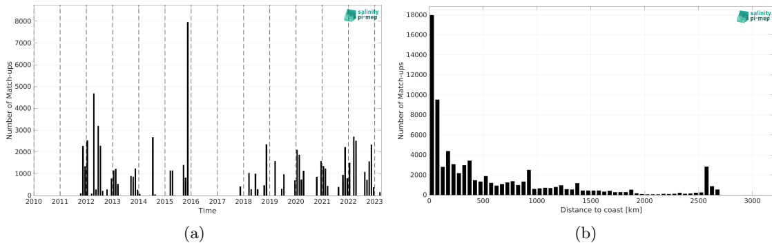
Figure 1: Number of match-ups between TSG (SAMOS) and SMAP SSS L4 OI v2 - 7 Days (ESR) SSS as a function of time (a) and as function of the distance to coast (b) over the Tropical Atlantic Ocean Pi-MEP region and for the full satellite product period.
