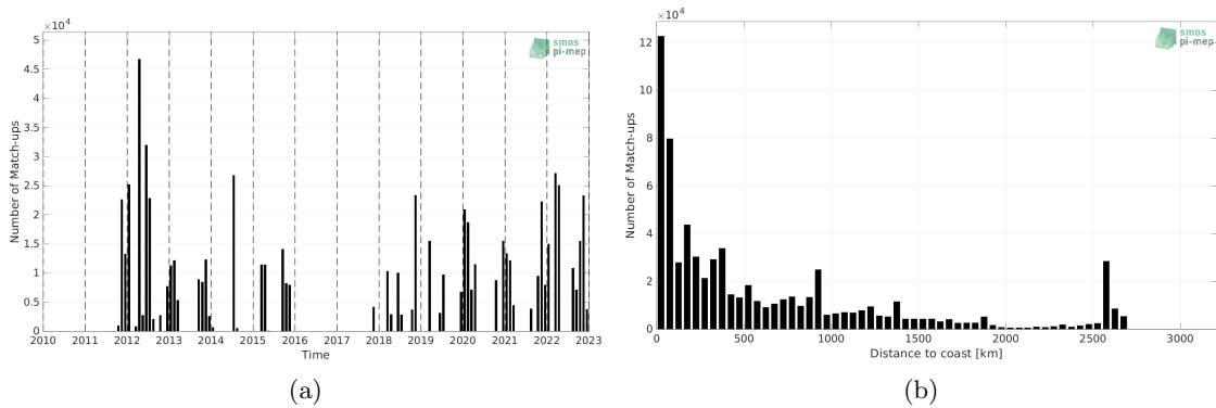
Figure 1: Number of match-ups between TSG (SAMOS) and SMAP SSS L4 OI v2 - 7 Days (ESR) SSS as a function of time (a) and as function of the distance to coast (b) over the Tropical Atlantic Ocean Pi-MEP region and for the full satellite product period.
