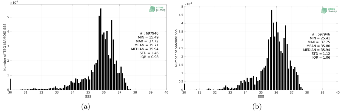
Figure 2: Histograms of SSS from TSG (SAMOS) (a) and SMAP SSS L4 OI v2 - 7 Days (ESR) (b) considering all match-up pairs per bins of 0.1 over the Tropical Atlantic Ocean Pi-MEP region and for the full satellite product period.
