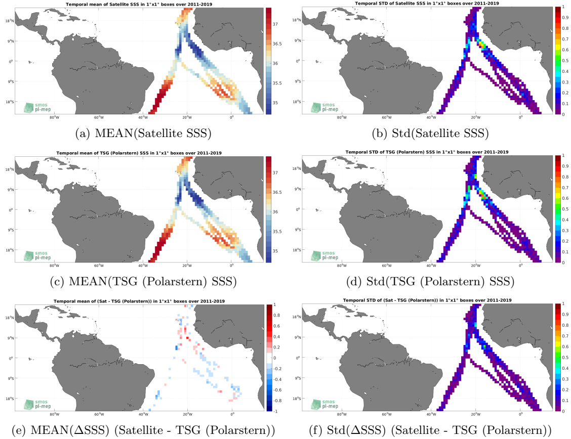
Figure 6: Temporal mean (left) and Std (right) of SSS from SMAP SSS L4 OI v2 - 7 Days (ESR) (top), TSG (Polarstern) (middle), and of \Delta\text{SSS} (Satellite - TSG (Polarstern)). Only match-up pairs are used to generate these maps.
