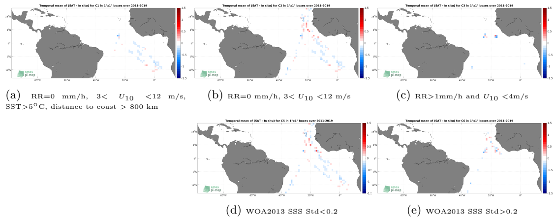
Figure 12: Temporal mean gridded over spatial boxes of size 1^\circ \times 1^\circ of \Delta SSS (SMAP SSS L4 OI v2 - 7 Days (ESR) - TSG (Polarstern)) for 5 different subdatasets corresponding to:RR=0 mm/h, 3 < U_{10} < 12 m/s, SST >5^\circ C, distance to coast > 800 km (a), RR=0 mm/h, 3 < U_{10} < 12 m/s (b), RR >1 mm/h and U_{10} < 4 m/s (c), WOA2013 SSS Std <0.2 (d), WOA2013 SSS Std >0.2 (e).
