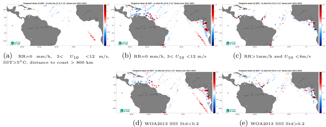
Figure 12: Temporal mean gridded over spatial boxes of size 1^\circ \times 1^\circ of \Delta\text{SSS} (SMAP SSS L4 OI v2 - 7 Days (ESR) - TSG (LEGOS-DM)) for 5 different subdatasets corresponding to:RR=0 mm/h, 3 < U_{10} < 12 m/s, SST >5^\circ\text{C} , distance to coast > 800 km (a), RR=0 mm/h, 3 < U_{10} < 12 m/s (b), RR >1 mm/h and U_{10} < 4 m/s (c), WOA2013 SSS Std <0.2 (d), WOA2013 SSS Std >0.2 (e).
