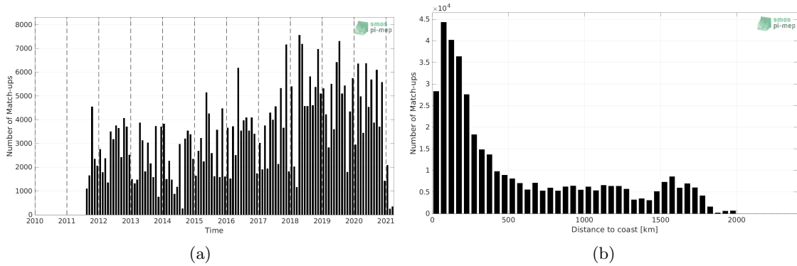
Figure 1: Number of match-ups between TSG (LEGOS-DM) and SMAP SSS L4 OI v2 - 7 Days (ESR) SSS as a function of time (a) and as function of the distance to coast (b) over the Tropical Atlantic Ocean Pi-MEP region and for the full satellite product period.
