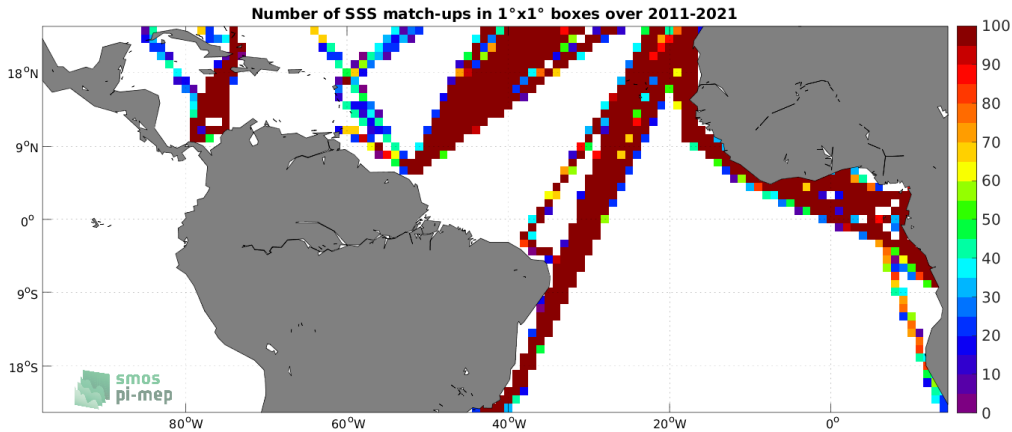
Figure 4: Number of SSS match-ups between TSG (LEGOS-DM) SSS and the SMAP SSS L4 OI v2 - 7 Days (ESR) SSS product for the Tropical Atlantic Ocean Pi-MEP region over 1^\circ \times 1^\circ boxes and for the full satellite product period.
