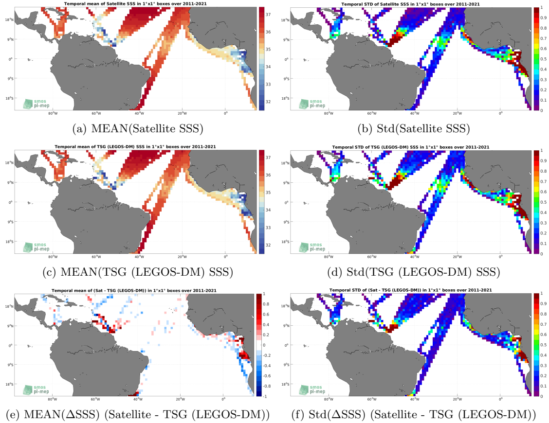
Figure 6: Temporal mean (left) and Std (right) of SSS from SMAP SSS L4 OI v2 - 7 Days (ESR) (top), TSG (LEGOS-DM) (middle), and of \Delta\text{SSS} (Satellite - TSG (LEGOS-DM)). Only match-up pairs are used to generate these maps.
