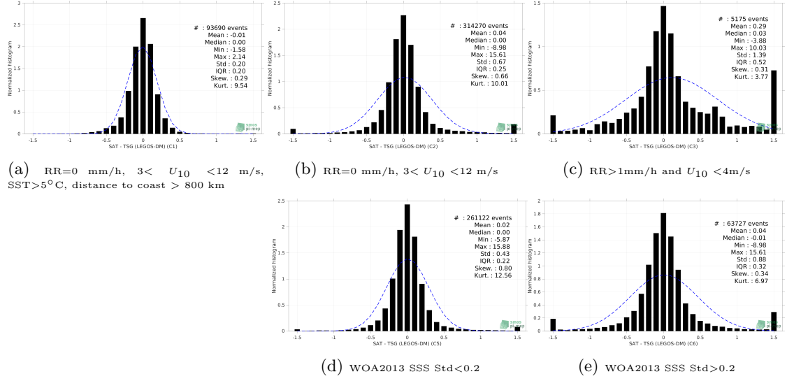
Figure 13: Normalized histogram of \Delta SSS (SMAP SSS L4 OI v2 - 7 Days (ESR) - TSG (LEGOS-DM)) for 5 different subdatasets corresponding to: RR=0 mm/h, 3 < U_{10} < 12 m/s, SST>5°C, distance to coast > 800 km (a), RR=0 mm/h, 3 < U_{10} < 12 m/s (b), RR>1mm/h and U_{10} < 4 m/s (c), WOA2013 SSS Std<0.2 (d), WOA2013 SSS Std>0.2 (e).
