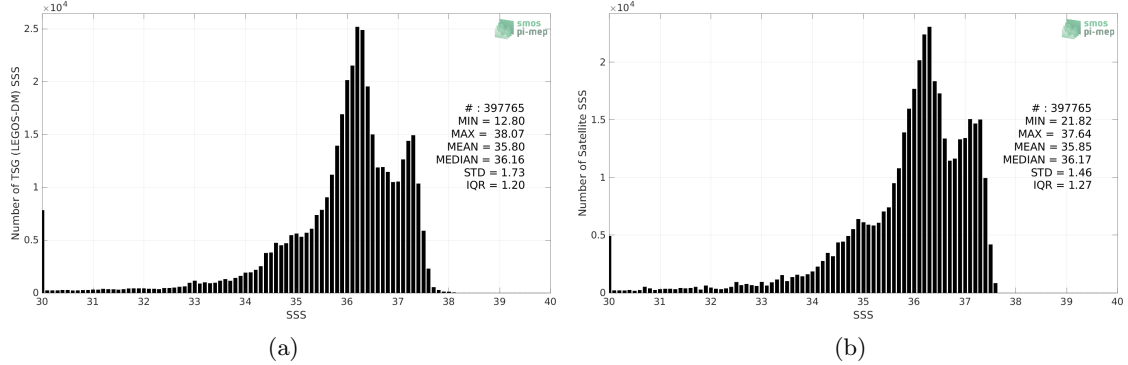
Figure 2: Histograms of SSS from TSG (LEGOS-DM) (a) and SMAP SSS L4 OI v2 - 7 Days (ESR) (b) considering all match-up pairs per bins of 0.1 over the Tropical Atlantic Ocean Pi-MEP region and for the full satellite product period.
