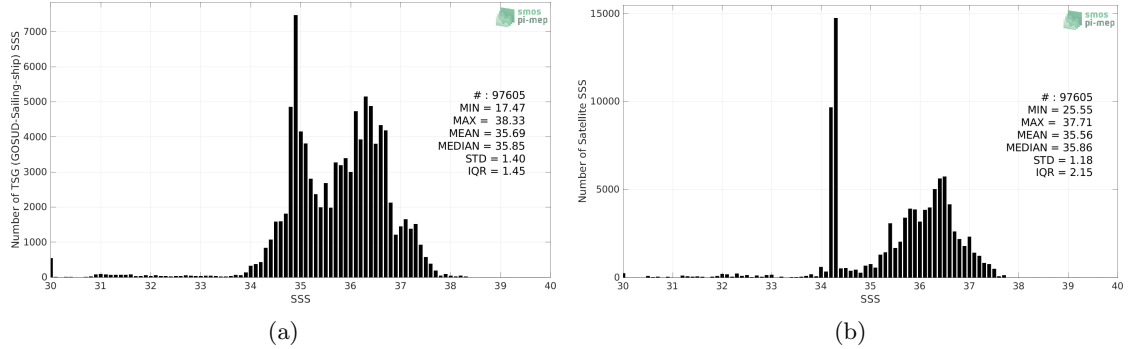
Figure 2: Histograms of SSS from TSG (GOSUD-Sailing-ship) (a) and SMAP SSS L4 OI v2 - 7 Days (ESR) (b) considering all match-up pairs per bins of 0.1 over the Tropical Atlantic Ocean Pi-MEP region and for the full satellite product period.
