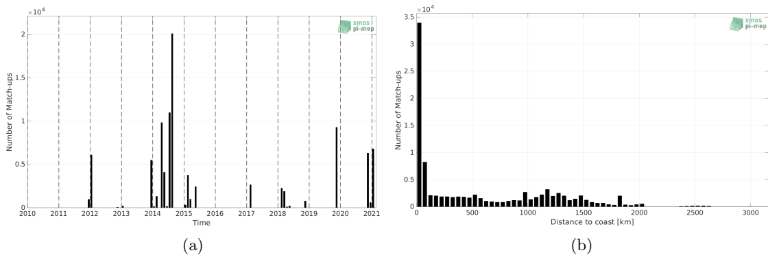
Figure 1: Number of match-ups between TSG (GOSUD-Sailing-ship) and SMAP SSS L4 OI v2 - 7 Days (ESR) SSS as a function of time (a) and as function of the distance to coast (b) over the Tropical Atlantic Ocean Pi-MEP region and for the full satellite product period.
