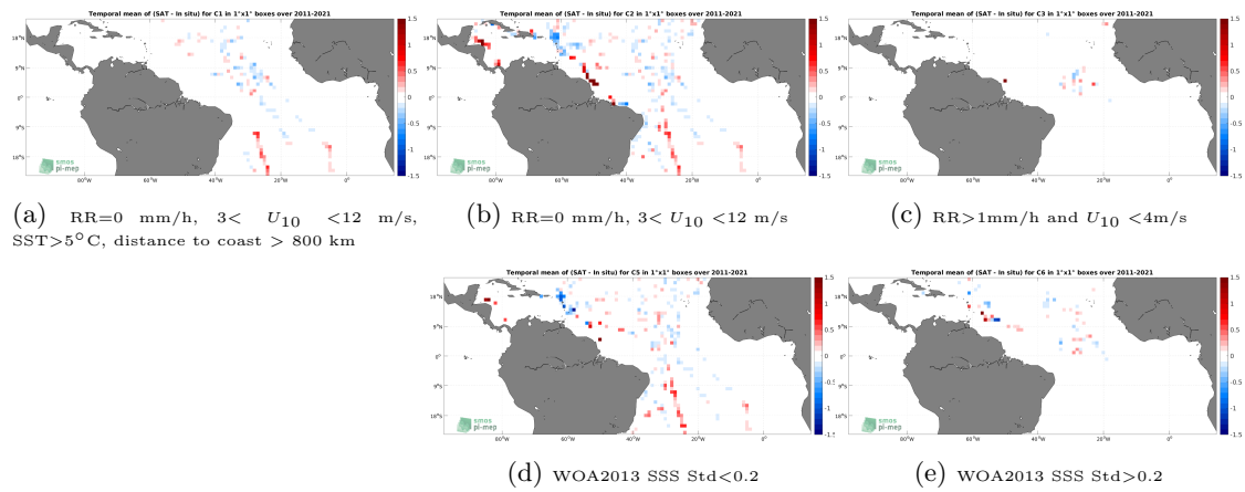
Figure 12: Temporal mean gridded over spatial boxes of size 1^\circ \times 1^\circ of \Delta SSS (SMAP SSS L4 OI v2 - 7 Days (ESR) - TSG (GOSUD-Sailing-ship)) for 5 different subdatasets corresponding to:RR=0 mm/h, 3 < U_{10} < 12 m/s, SST>5°C, distance to coast > 800 km (a), RR=0 mm/h, 3 < U_{10} < 12 m/s (b), RR>1mm/h and U_{10} < 4 m/s (c), WOA2013 SSS Std<0.2 (d), WOA2013 SSS Std>0.2 (e).
