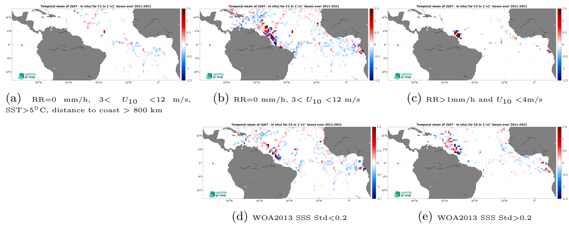
Figure 12: Temporal mean gridded over spatial boxes of size 1^\circ \times 1^\circ of \Delta\text{SSS} (SMAP SSS L4 OI v2 - 7 Days (ESR) - TSG (GOSUD-Research-vessel)) for 5 different subdatasets corresponding to:RR=0 mm/h, 3 < U_{10} < 12 m/s, SST>5°C, distance to coast > 800 km (a), RR=0 mm/h, 3 < U_{10} < 12 m/s (b), RR>1mm/h and U_{10} < 4 m/s (c), WOA2013 SSS Std<0.2 (d), WOA2013 SSS Std>0.2 (e).
