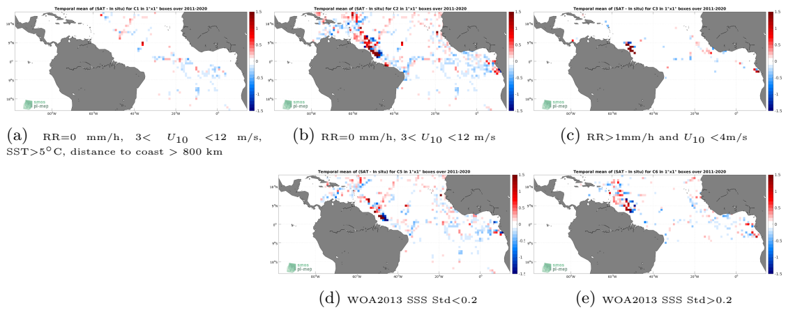
Figure 12: Temporal mean gridded over spatial boxes of size 1^\circ \times 1^\circ of \Delta SSS (SMAP SSS L4 OI v2 - 7 Days (ESR) - TSG (GOSUD-Research-vessel)) for 5 different subdatasets corresponding to:RR=0 mm/h, 3 < U_{10} < 12 m/s, SST>5°C, distance to coast > 800 km (a), RR=0 mm/h, 3 < U_{10} < 12 m/s (b), RR>1mm/h and U_{10} < 4 m/s (c), WOA2013 SSS Std<0.2 (d), WOA2013 SSS Std>0.2 (e).
