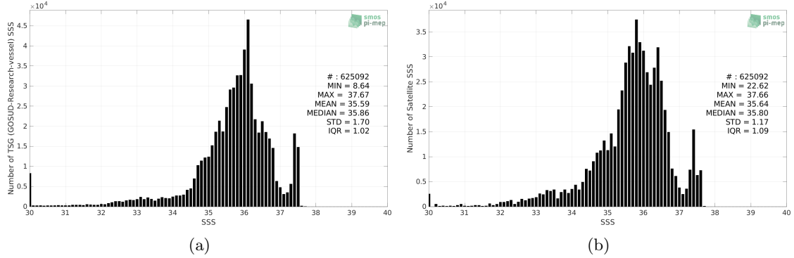
Figure 2: Histograms of SSS from TSG (GOSUD-Research-vessel) (a) and SMAP SSS L4 OI v2 - 7 Days (ESR) (b) considering all match-up pairs per bins of 0.1 over the Tropical Atlantic Ocean Pi-MEP region and for the full satellite product period.
