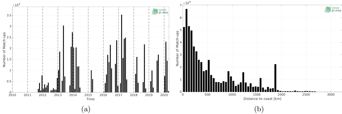
Figure 1: Number of match-ups between TSG (GOSUD-Research-vessel) and SMAP SSS L4 OI v2 - 7 Days (ESR) SSS as a function of time (a) and as function of the distance to coast (b) over the Tropical Atlantic Ocean Pi-MEP region and for the full satellite product period.
