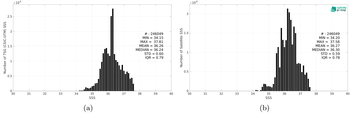
Figure 2: Histograms of SSS from TSG (CSIC-UTM) (a) and SMAP SSS L4 OI v2 - 7 Days (ESR) (b) considering all match-up pairs per bins of 0.1 over the Tropical Atlantic Ocean Pi-MEP region and for the full satellite product period.
