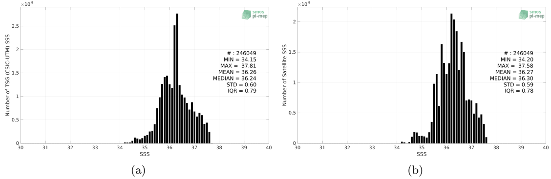
Figure 2: Histograms of SSS from TSG (CSIC-UTM) (a) and SMAP SSS L4 OI v2 - 7 Days (ESR) (b) considering all match-up pairs per bins of 0.1 over the Tropical Atlantic Ocean Pi-MEP region and for the full satellite product period.
