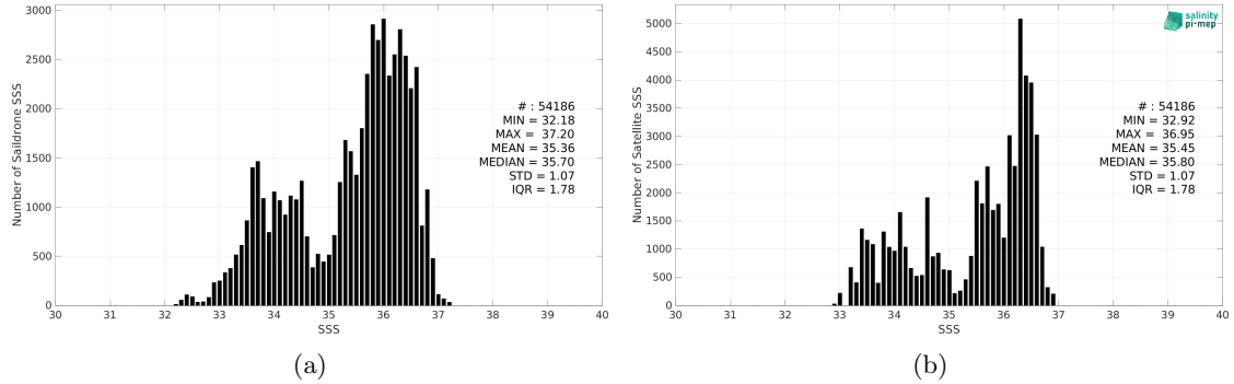
Figure 2: Histograms of SSS from Saildrone (a) and SMAP SSS L4 OI v2 - 7 Days (ESR) (b) considering all match-up pairs per bins of 0.1 over the Tropical Atlantic Ocean Pi-MEP region and for the full satellite product period.
