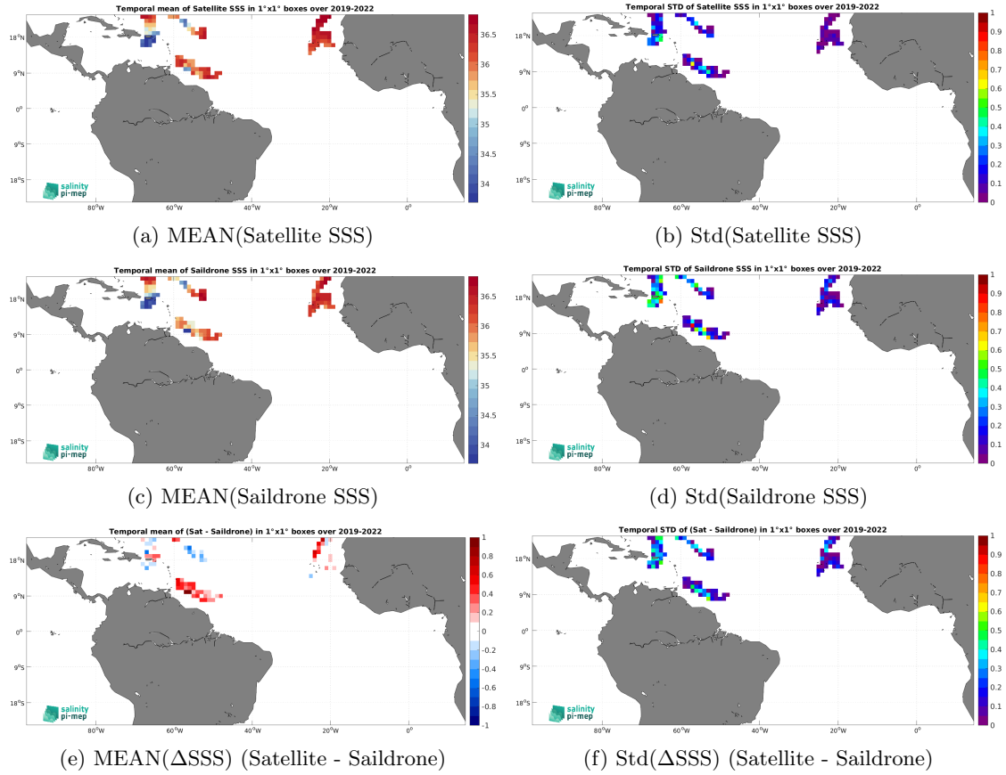
Figure 6: Temporal mean (left) and Std (right) of SSS from SMAP SSS L4 OI v2 - 7 Days (ESR) (top), Saildrone (middle), and of \Delta\text{SSS} (Satellite - Saildrone). Only match-up pairs are used to generate these maps.
