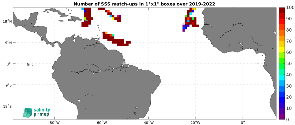
Figure 4: Number of SSS match-ups between Saildrone SSS and the SMAP SSS L4 OI v2 - 7 Days (ESR) SSS product for the Tropical Atlantic Ocean Pi-MEP region over 1^\circ \times 1^\circ boxes and for the full satellite product period.
