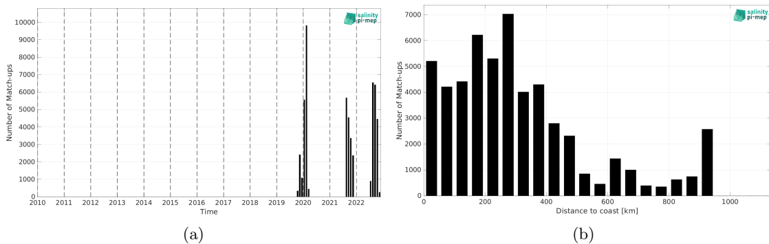
Figure 1: Number of match-ups between Saildrone and SMAP SSS L4 OI v2 - 7 Days (ESR) SSS as a function of time (a) and as function of the distance to coast (b) over the Tropical Atlantic Ocean Pi-MEP region and for the full satellite product period.
