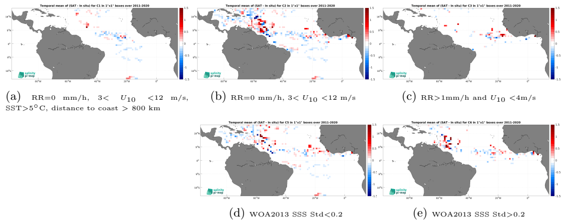
Figure 11: Temporal mean gridded over spatial boxes of size 1^\circ \times 1^\circ of \Delta\text{SSS} (SMAP SSS L4 OI v2 - 7 Days (ESR) - Surface drifters) for 5 different subdatasets corresponding to:RR=0 mm/h, 3 < U_{10} < 12 m/s, SST >5^\circ\text{C} , distance to coast > 800 km (a), RR=0 mm/h, 3 < U_{10} < 12 m/s (b), RR >1 mm/h and U_{10} < 4 m/s (c), WOA2013 SSS Std <0.2 (d), WOA2013 SSS Std >0.2 (e).
