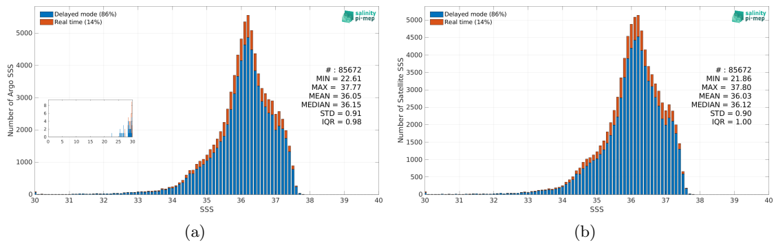
Figure 2: Histograms of SSS from Argo (a) and SMAP SSS L4 OI v2 - 7 Days (ESR) (b) considering all match-up pairs per bins of 0.1 over the Tropical Atlantic Ocean Pi-MEP region and for the full satellite product period.
