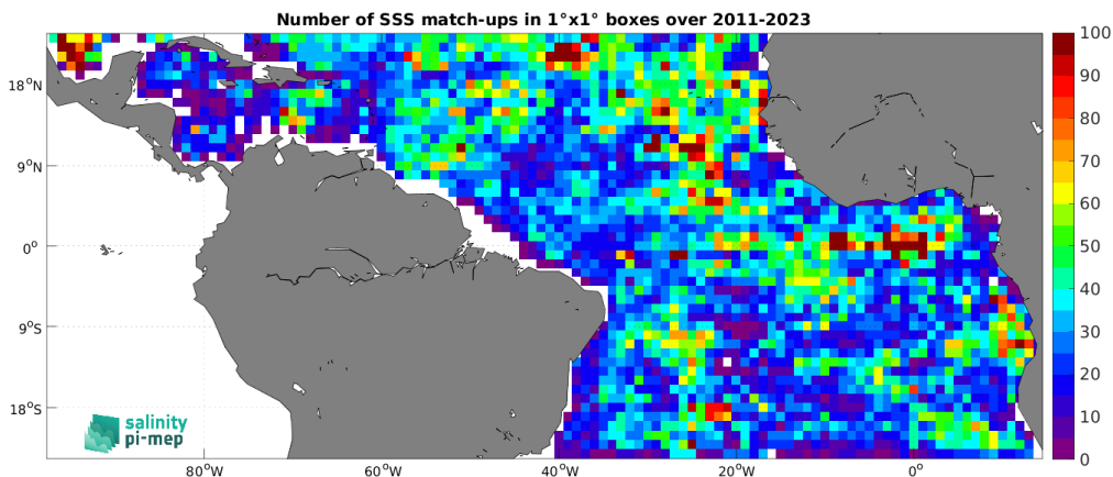
Figure 4: Number of SSS match-ups between Argo SSS and the SMAP SSS L4 OI v2 - 7 Days (ESR) SSS product for the Tropical Atlantic Ocean Pi-MEP region over 1^\circ \times 1^\circ boxes and for the full satellite product period.
