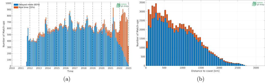
Figure 1: Number of match-ups between Argo and SMAP SSS L4 OI v2 - 7 Days (ESR) SSS as a function of time (a) and as function of the distance to coast (b) over the Tropical Atlantic Ocean Pi-MEP region and for the full satellite product period.
