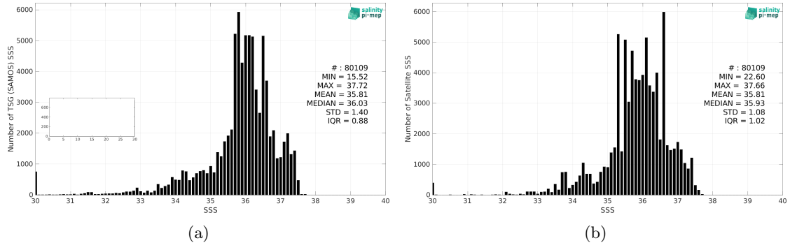
Figure 2: Histograms of SSS from TSG (SAMOS) (a) and SMAP SSS L4 OI v2 - Monthly (IPRC) (b) considering all match-up pairs per bins of 0.1 over the Tropical Atlantic Ocean Pi-MEP region and for the full satellite product period.
