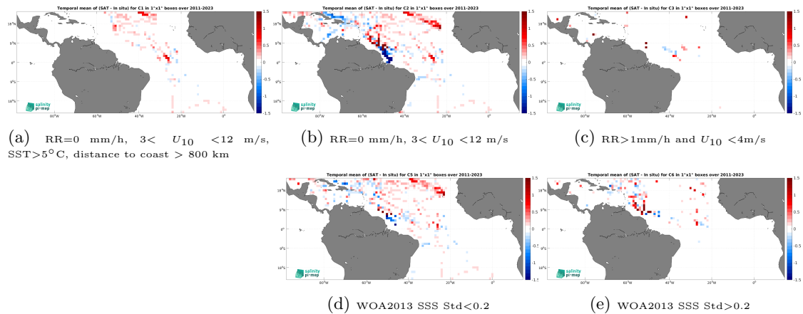
Figure 12: Temporal mean gridded over spatial boxes of size 1^\circ \times 1^\circ of \Delta\text{SSS} (SMAP SSS L4 OI v2 - Monthly (IPRC) - TSG (SAMOS)) for 5 different subdatasets corresponding to:RR=0 mm/h, 3 < U_{10} < 12 m/s, SST >5^\circ\text{C} , distance to coast > 800 km (a), RR=0 mm/h, 3 < U_{10} < 12 m/s (b), RR >1 mm/h and U_{10} < 4 m/s (c), WOA2013 SSS Std <0.2 (d), WOA2013 SSS Std >0.2 (e).
