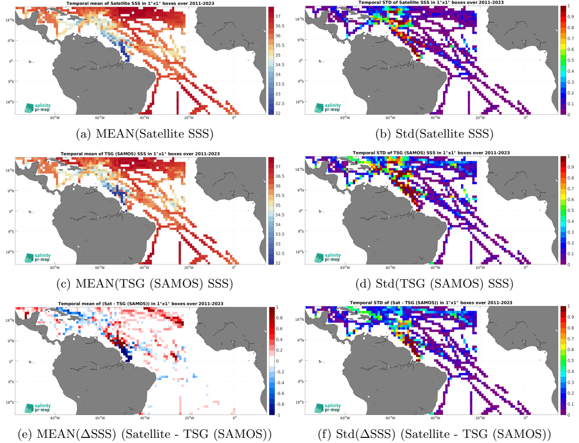
Figure 6: Temporal mean (left) and Std (right) of SSS from SMAP SSS L4 OI v2 - Monthly (IPRC) (top), TSG (SAMOS) (middle), and of \Delta\text{SSS}(\text{Satellite} - \text{TSG}(\text{SAMOS})) . Only match-up pairs are used to generate these maps.
