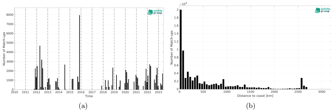
Figure 1: Number of match-ups between TSG (SAMOS) and SMAP SSS L4 OI v2 - Monthly (IPRC) SSS as a function of time (a) and as function of the distance to coast (b) over the Tropical Atlantic Ocean Pi-MEP region and for the full satellite product period.
