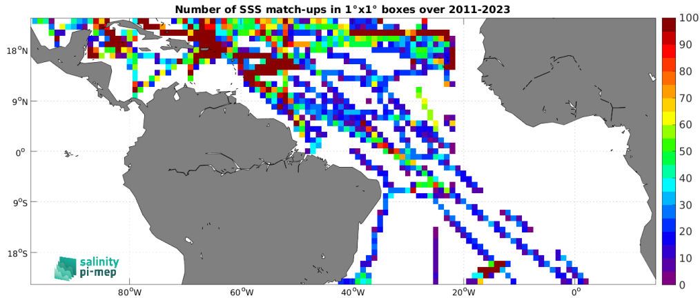
Figure 4: Number of SSS match-ups between TSG (SAMOS) SSS and the SMAP SSS L4 OI v2 - Monthly (IPRC) SSS product for the Tropical Atlantic Ocean Pi-MEP region over 1^\circ \times 1^\circ boxes and for the full satellite product period.
