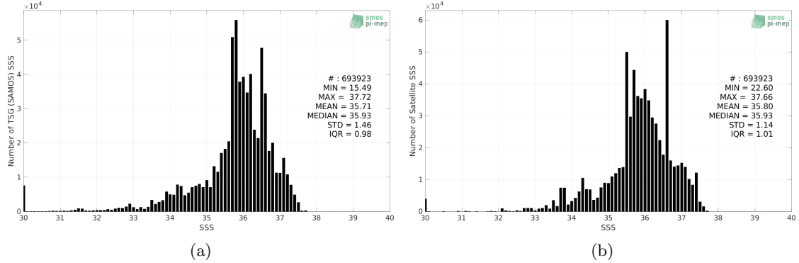
Figure 2: Histograms of SSS from TSG (SAMOS) (a) and SMAP SSS L4 OI v2 - Monthly (IPRC) (b) considering all match-up pairs per bins of 0.1 over the Tropical Atlantic Ocean Pi-MEP region and for the full satellite product period.
