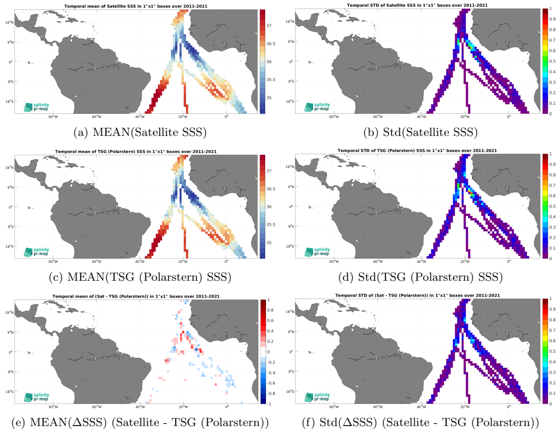
Figure 6: Temporal mean (left) and Std (right) of SSS from SMAP SSS L4 OI v2 - Monthly (IPRC) (top), TSG (Polarstern) (middle), and of \Delta SSS (Satellite - TSG (Polarstern)). Only match-up pairs are used to generate these maps.
