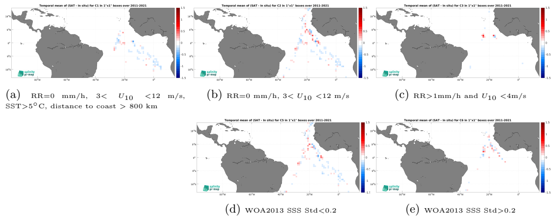
Figure 12: Temporal mean gridded over spatial boxes of size 1^\circ \times 1^\circ of \Delta\text{SSS} (SMAP SSS L4 OI v2 - Monthly (IPRC) - TSG (Polarstern)) for 5 different subdatasets corresponding to:RR=0 mm/h, 3 < U_{10} < 12 m/s, SST >5^\circ\text{C} , distance to coast > 800 km (a), RR=0 mm/h, 3 < U_{10} < 12 m/s (b), RR >1 mm/h and U_{10} < 4 m/s (c), WOA2013 SSS Std <0.2 (d), WOA2013 SSS Std >0.2 (e).
