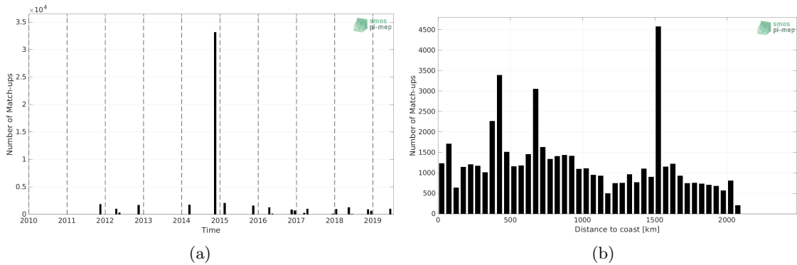
Figure 1: Number of match-ups between TSG (Polarstern) and SMAP SSS L4 OI v2 - Monthly (IPRC) SSS as a function of time (a) and as function of the distance to coast (b) over the Tropical Atlantic Ocean Pi-MEP region and for the full satellite product period.
