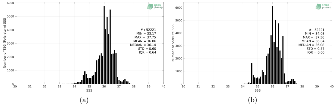
Figure 2: Histograms of SSS from TSG (Polarstern) (a) and SMAP SSS L4 OI v2 - Monthly (IPRC) (b) considering all match-up pairs per bins of 0.1 over the Tropical Atlantic Ocean Pi-MEP region and for the full satellite product period.
