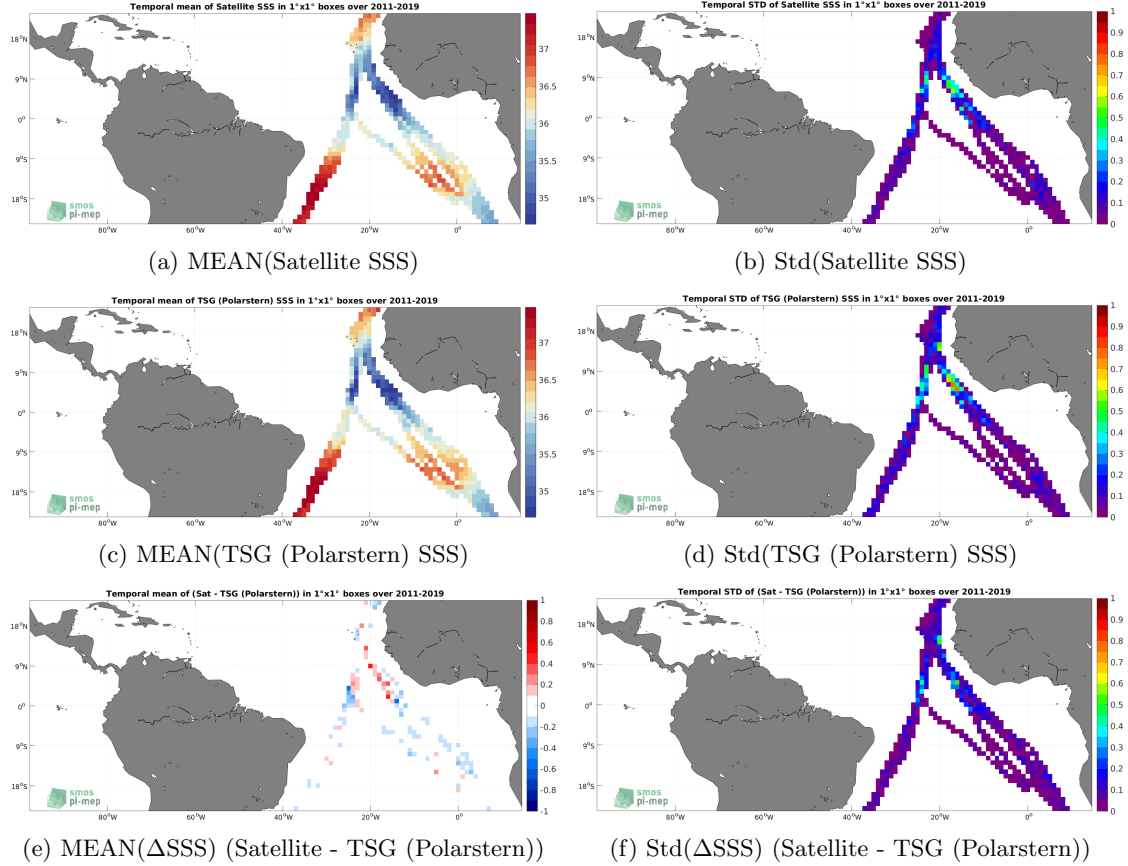
Figure 6: Temporal mean (left) and Std (right) of SSS from SMAP SSS L4 OI v2 - Monthly (IPRC) (top), TSG (Polarstern) (middle), and of \Delta\text{SSS}(\text{Satellite} - \text{TSG}(\text{Polarstern})) . Only match-up pairs are used to generate these maps.
