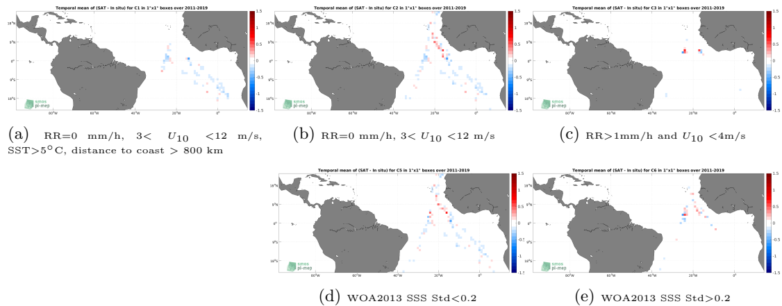
Figure 12: Temporal mean gridded over spatial boxes of size 1^\circ \times 1^\circ of \Delta SSS (SMAP SSS L4 OI v2 - Monthly (IPRC) - TSG (Polarstern)) for 5 different subdatasets corresponding to:RR=0 mm/h, 3 < U_{10} < 12 m/s, SST >5^\circ\text{C} , distance to coast > 800 km (a), RR=0 mm/h, 3 < U_{10} < 12 m/s (b), RR >1 mm/h and U_{10} < 4 m/s (c), WOA2013 SSS Std <0.2 (d), WOA2013 SSS Std >0.2 (e).
