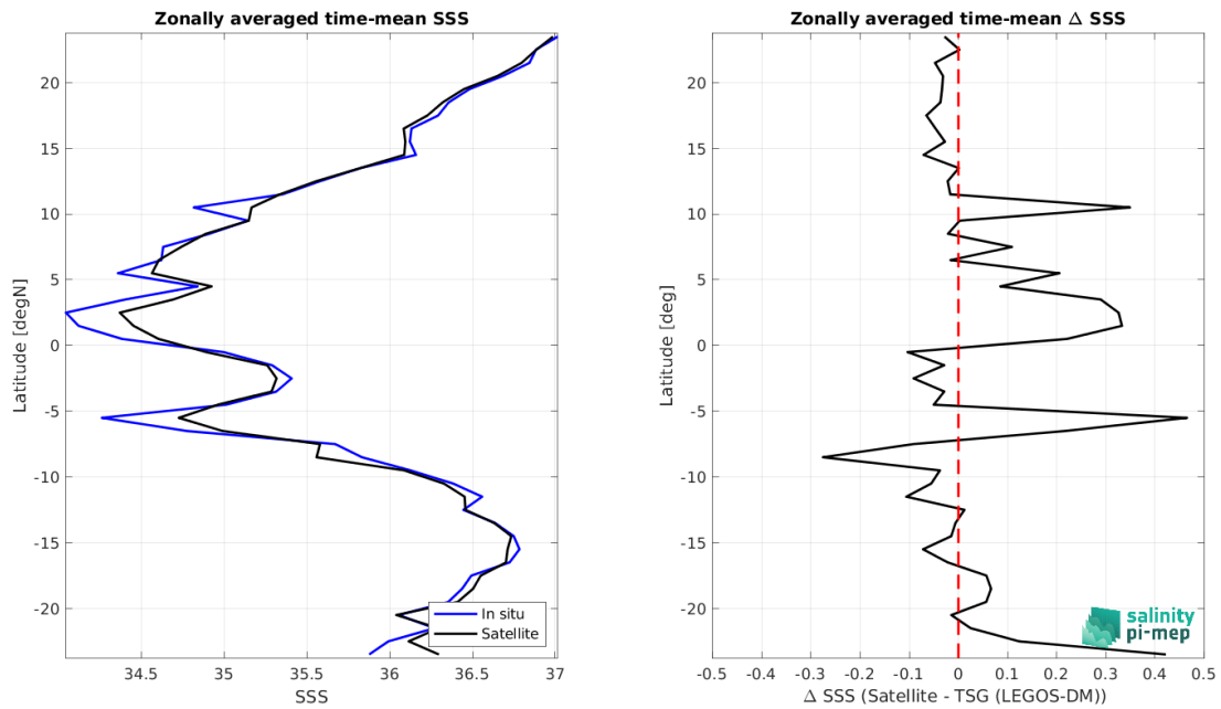
Figure 8: Left panel: Zonal mean SSS from SMAP SSS L4 OI v2 - Monthly (IPRC) satellite product (black) and from TSG (LEGOS-DM) (blue). Right panel: Zonal mean of \Delta SSS (Satellite - TSG (LEGOS-DM)) for all the collected Pi-MEP match-up pairs estimated over the full satellite product period.
