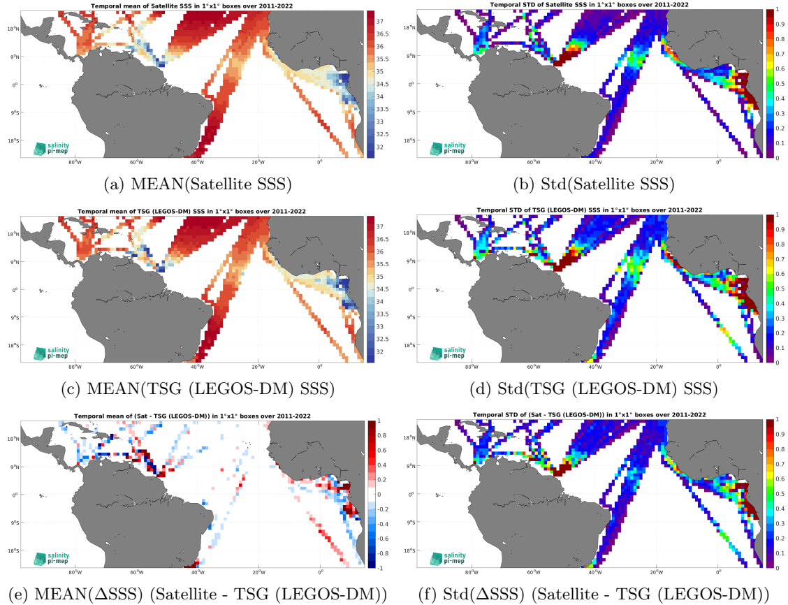
Figure 6: Temporal mean (left) and Std (right) of SSS from SMAP SSS L4 OI v2 - Monthly (IPRC) (top), TSG (LEGOS-DM) (middle), and of \Delta\text{SSS} (Satellite - TSG (LEGOS-DM)). Only match-up pairs are used to generate these maps.
