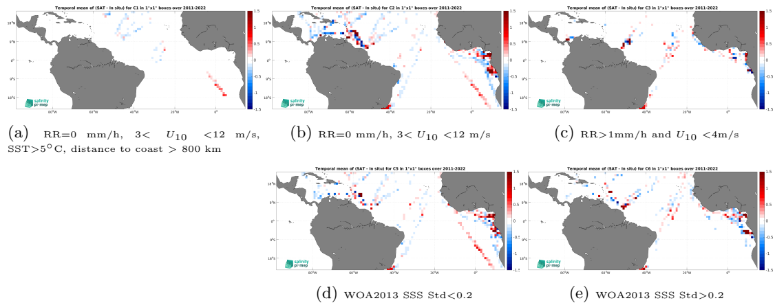
Figure 12: Temporal mean gridded over spatial boxes of size 1^\circ \times 1^\circ of \Delta\text{SSS} (SMAP SSS L4 OI v2 - Monthly (IPRC) - TSG (LEGOS-DM)) for 5 different subdatasets corresponding to:RR=0 mm/h, 3 < U_{10} < 12 m/s, SST >5^\circ\text{C} , distance to coast > 800 km (a), RR=0 mm/h, 3 < U_{10} < 12 m/s (b), RR >1 mm/h and U_{10} < 4 m/s (c), WOA2013 SSS Std <0.2 (d), WOA2013 SSS Std >0.2 (e).
