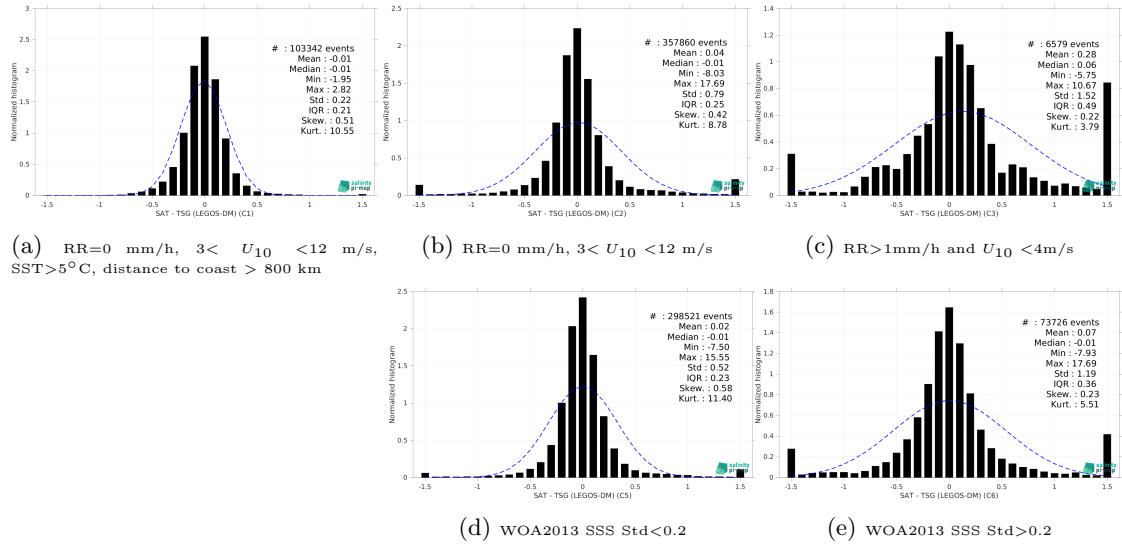
Figure 13: Normalized histogram of \Delta SSS (SMAP SSS L4 OI v2 - Monthly (IPRC) - TSG (LEGOS-DM)) for 5 different subdatasets corresponding to: RR=0 mm/h, 3 < U_{10} < 12 m/s, SST>5°C, distance to coast > 800 km (a), RR=0 mm/h, 3 < U_{10} < 12 m/s (b), RR>1mm/h and U_{10} < 4 m/s (c), WOA2013 SSS Std<0.2 (d), WOA2013 SSS Std>0.2 (e).
