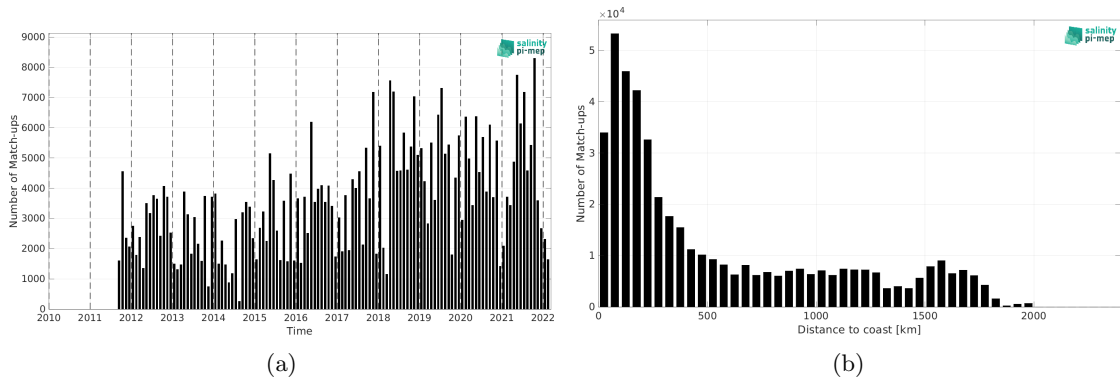
Figure 1: Number of match-ups between TSG (LEGOS-DM) and SMAP SSS L4 OI v2 - Monthly (IPRC) SSS as a function of time (a) and as function of the distance to coast (b) over the Tropical Atlantic Ocean Pi-MEP region and for the full satellite product period.
