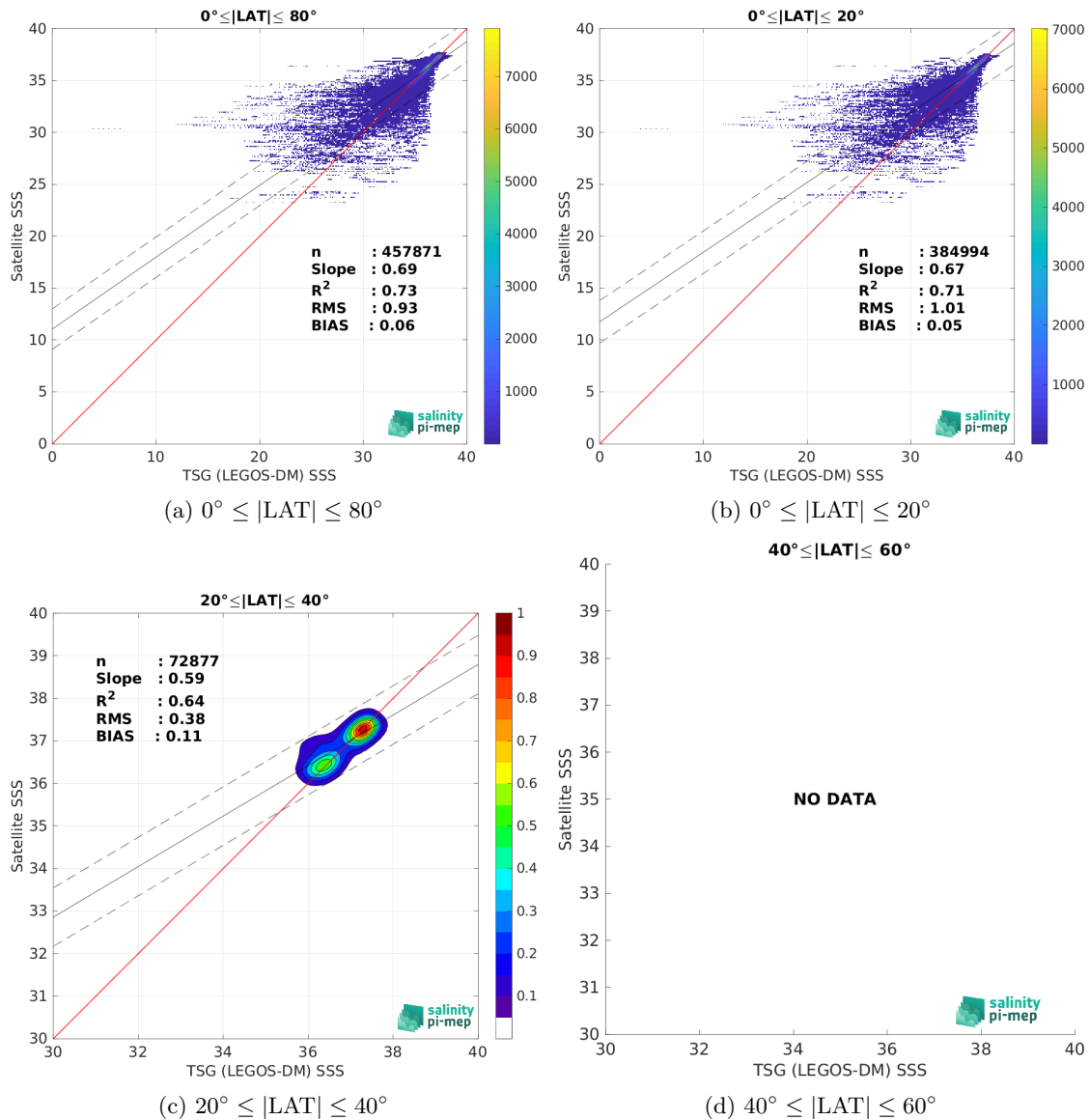
Figure 9: Contour maps of the concentration of SMAP SSS L4 OI v2 - Monthly (IPRC) SSS (y-axis) versus TSG (LEGOS-DM) SSS (x-axis) at match-up pairs for different latitude bands. For each plot, the red line shows x=y . The black thin and dashed lines indicate a linear fit through the data cloud and the \pm 95\% confidence levels, respectively. The number match-up pairs n , the slope and R^2 coefficient of the linear fit, the root mean square (RMS) and the mean bias between satellite and in situ data are indicated for each latitude band in each plots.
