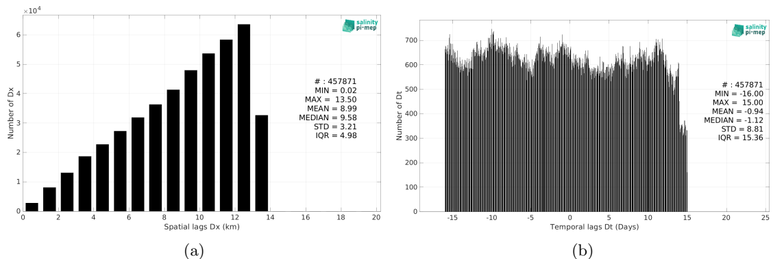
Figure 5: Histograms of the spatial (a) and temporal (b) lags between the location/time of the TSG (LEGOS-DM) measurement and the date of the corresponding SMAP SSS L4 OI v2 - Monthly (IPRC) SSS pixel.
