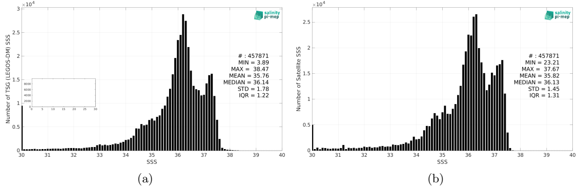
Figure 2: Histograms of SSS from TSG (LEGOS-DM) (a) and SMAP SSS L4 OI v2 - Monthly (IPRC) (b) considering all match-up pairs per bins of 0.1 over the Tropical Atlantic Ocean Pi-MEP region and for the full satellite product period.
