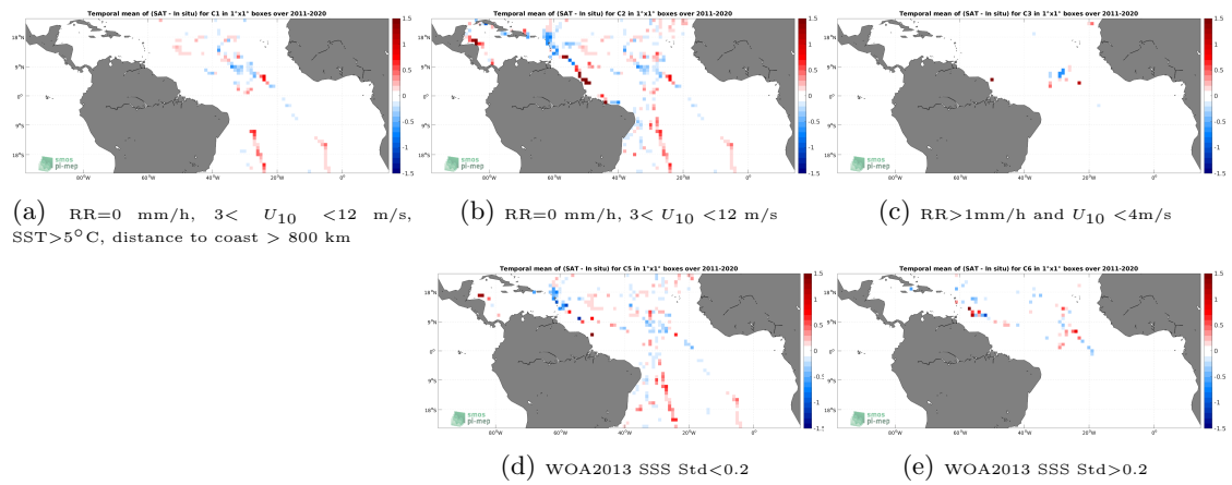
Figure 12: Temporal mean gridded over spatial boxes of size 1^\circ \times 1^\circ of \Delta SSS (SMAP SSS L4 OI v2 - Monthly (IPRC) - TSG (GOSUD-Sailing-ship)) for 5 different subdatasets corresponding to:RR=0 mm/h, 3 < U_{10} < 12 m/s, SST>5°C, distance to coast > 800 km (a), RR=0 mm/h, 3 < U_{10} < 12 m/s (b), RR>1mm/h and U_{10} < 4 m/s (c), WOA2013 SSS Std<0.2 (d), WOA2013 SSS Std>0.2 (e).
