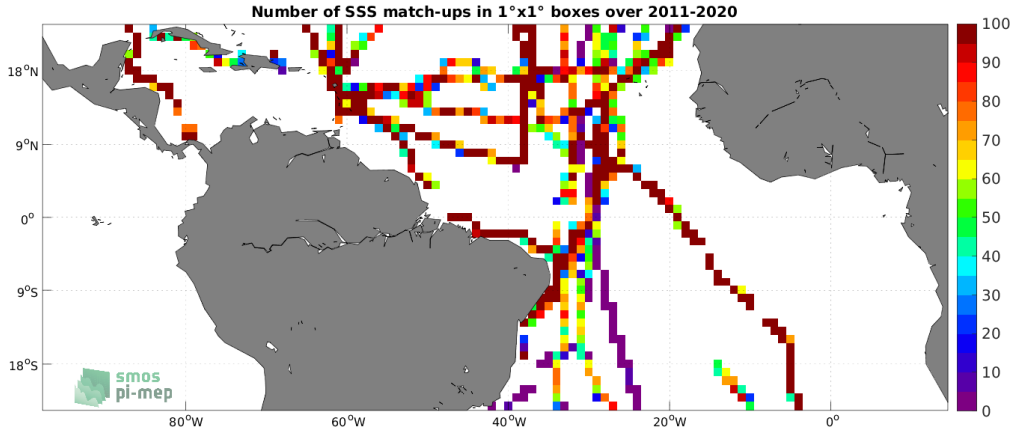
Figure 4: Number of SSS match-ups between TSG (GOSUD-Sailing-ship) SSS and the SMAP SSS L4 OI v2 - Monthly (IPRC) SSS product for the Tropical Atlantic Ocean Pi-MEP region over 1^\circ \times 1^\circ boxes and for the full satellite product period.
