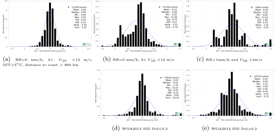
Figure 13: Normalized histogram of \Delta SSS (SMAP SSS L4 OI v2 - Monthly (IPRC) - TSG (GOSUD-Sailing-ship)) for 5 different subdatasets corresponding to: RR=0 mm/h, 3 < U_{10} < 12 m/s, SST > 5°C, distance to coast > 800 km (a), RR=0 mm/h, 3 < U_{10} < 12 m/s (b), RR > 1mm/h and U_{10} < 4 m/s (c), WOA2013 SSS Std < 0.2 (d), WOA2013 SSS Std > 0.2 (e).
