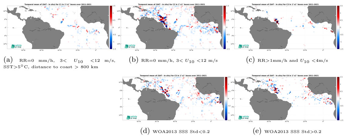
Figure 12: Temporal mean gridded over spatial boxes of size 1^\circ \times 1^\circ of \Delta\text{SSS} (SMAP SSS L4 OI v2 - Monthly (IPRC) - TSG (GOSUD-Research-vessel)) for 5 different subdatasets corresponding to:RR=0 mm/h, 3 < U_{10} < 12 m/s, SST>5°C, distance to coast > 800 km (a), RR=0 mm/h, 3 < U_{10} < 12 m/s (b), RR>1mm/h and U_{10} < 4 m/s (c), WOA2013 SSS Std<0.2 (d), WOA2013 SSS Std>0.2 (e).
