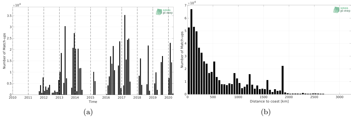
Figure 1: Number of match-ups between TSG (GOSUD-Research-vessel) and SMAP SSS L4 OI v2 - Monthly (IPRC) SSS as a function of time (a) and as function of the distance to coast (b) over the Tropical Atlantic Ocean Pi-MEP region and for the full satellite product period.
