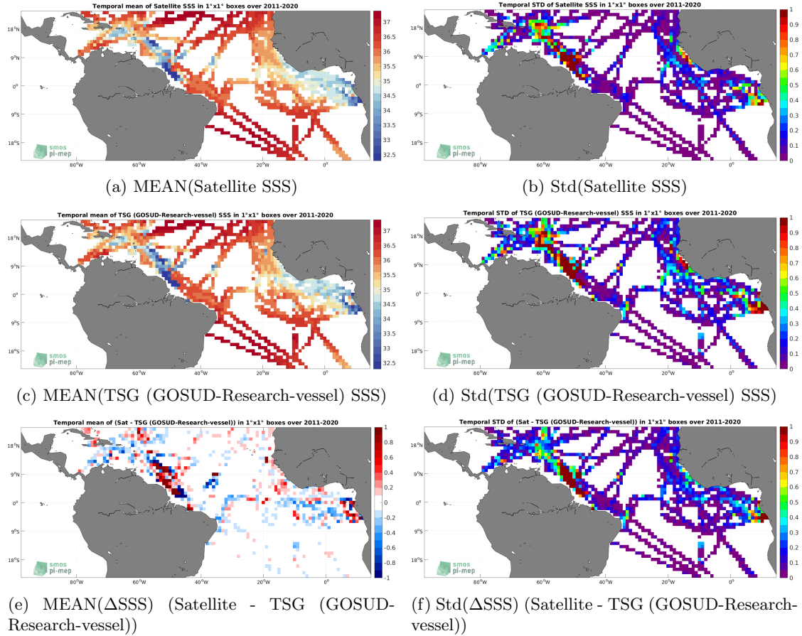
Figure 6: Temporal mean (left) and Std (right) of SSS from SMAP SSS L4 OI v2 - Monthly (IPRC) (top), TSG (GOSUD-Research-vessel) (middle), and of \Delta\text{SSS} (Satellite - TSG (GOSUD-Research-vessel)). Only match-up pairs are used to generate these maps.
