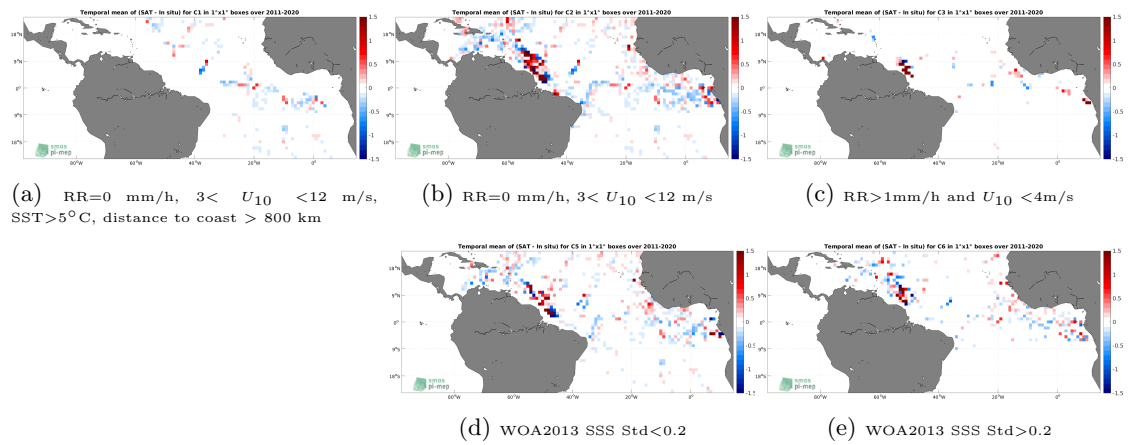
Figure 12: Temporal mean gridded over spatial boxes of size 1^\circ \times 1^\circ of \Delta SSS (SMAP SSS L4 OI v2 - Monthly (IPRC) - TSG (GOSUD-Research-vessel)) for 5 different subdatasets corresponding to:RR=0 mm/h, 3 < U_{10} < 12 m/s, SST>5°C, distance to coast > 800 km (a), RR=0 mm/h, 3 < U_{10} < 12 m/s (b), RR>1mm/h and U_{10} < 4 m/s (c), WOA2013 SSS Std<0.2 (d), WOA2013 SSS Std>0.2 (e).
