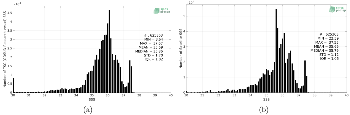
Figure 2: Histograms of SSS from TSG (GOSUD-Research-vessel) (a) and SMAP SSS L4 OI v2 - Monthly (IPRC) (b) considering all match-up pairs per bins of 0.1 over the Tropical Atlantic Ocean Pi-MEP region and for the full satellite product period.
