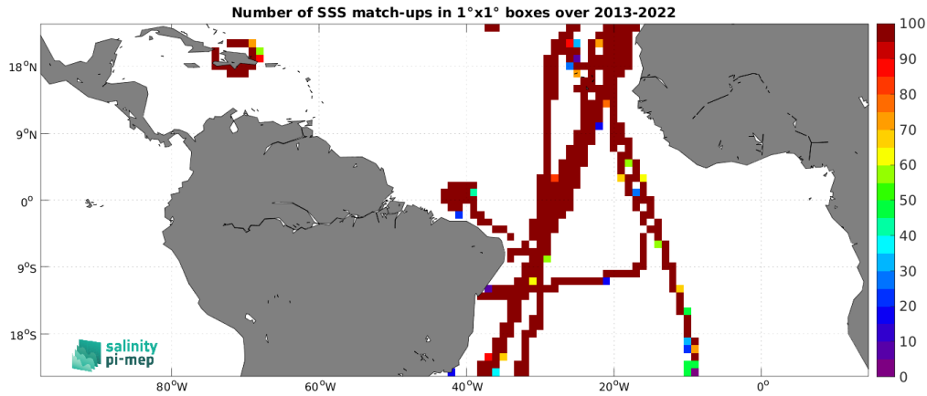
Figure 4: Number of SSS match-ups between TSG (CSIC-UTM) SSS and the SMAP SSS L4 OI v2 - Monthly (IPRC) SSS product for the Tropical Atlantic Ocean Pi-MEP region over 1^\circ \times 1^\circ boxes and for the full satellite product period.
