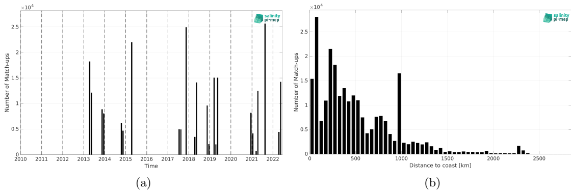
Figure 1: Number of match-ups between TSG (CSIC-UTM) and SMAP SSS L4 OI v2 - Monthly (IPRC) SSS as a function of time (a) and as function of the distance to coast (b) over the Tropical Atlantic Ocean Pi-MEP region and for the full satellite product period.
