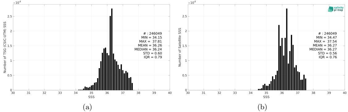
Figure 2: Histograms of SSS from TSG (CSIC-UTM) (a) and SMAP SSS L4 OI v2 - Monthly (IPRC) (b) considering all match-up pairs per bins of 0.1 over the Tropical Atlantic Ocean Pi-MEP region and for the full satellite product period.
