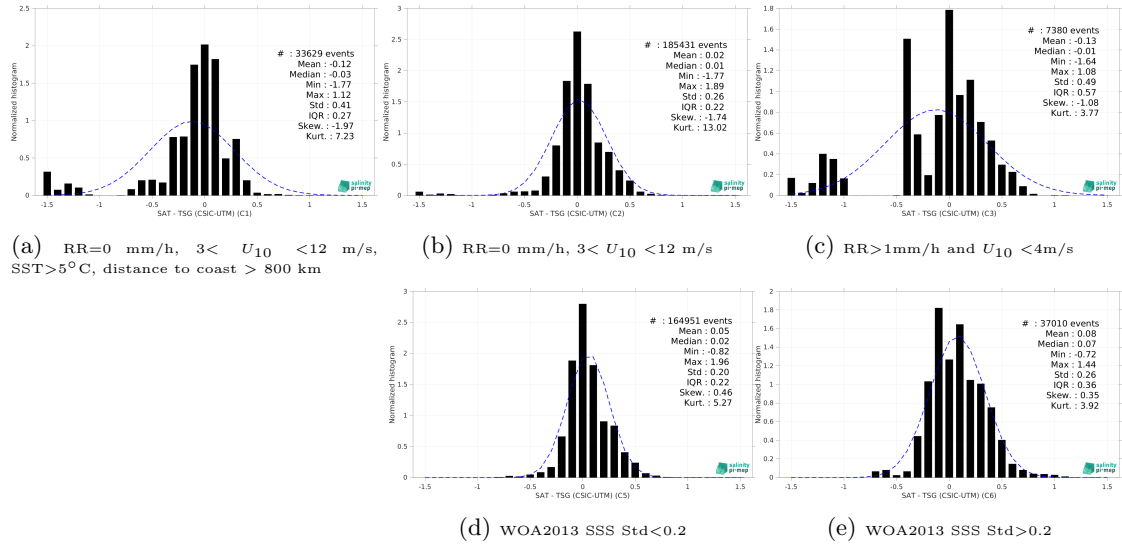
Figure 13: Normalized histogram of \Delta\text{SSS} (SMAP SSS L4 OI v2 - Monthly (IPRC) - TSG (CSIC-UTM)) for 5 different subdatasets corresponding to: RR=0 mm/h, 3 < U_{10} < 12 m/s, SST>5°C, distance to coast > 800 km (a), RR=0 mm/h, 3 < U_{10} < 12 m/s (b), RR>1mm/h and U_{10} < 4 m/s (c), WOA2013 SSS Std<0.2 (d), WOA2013 SSS Std>0.2 (e).
