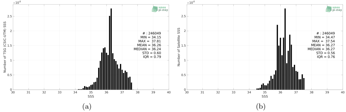
Figure 2: Histograms of SSS from TSG (CSIC-UTM) (a) and SMAP SSS L4 OI v2 - Monthly (IPRC) (b) considering all match-up pairs per bins of 0.1 over the Tropical Atlantic Ocean Pi-MEP region and for the full satellite product period.
