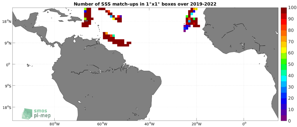
Figure 4: Number of SSS match-ups between Saildrone SSS and the SMAP SSS L4 OI v2 - Monthly (IPRC) SSS product for the Tropical Atlantic Ocean Pi-MEP region over 1^\circ \times 1^\circ boxes and for the full satellite product period.
