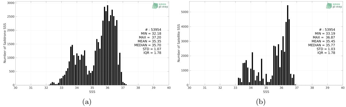
Figure 2: Histograms of SSS from Saildrone (a) and SMAP SSS L4 OI v2 - Monthly (IPRC) (b) considering all match-up pairs per bins of 0.1 over the Tropical Atlantic Ocean Pi-MEP region and for the full satellite product period.
