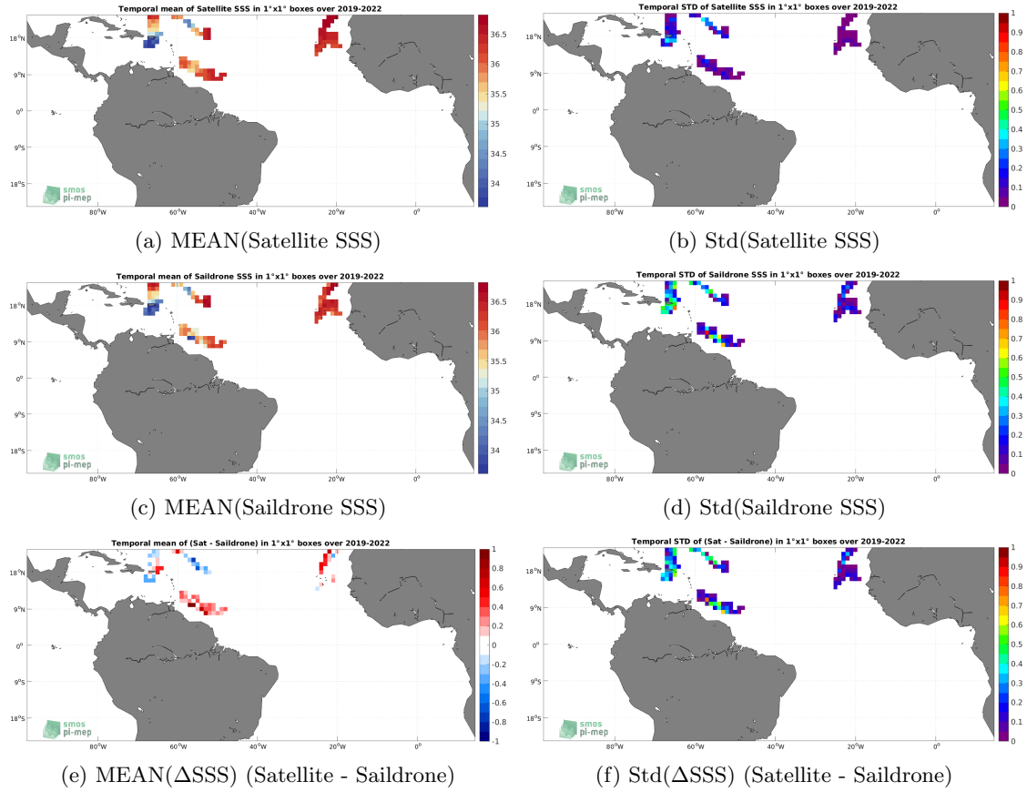
Figure 6: Temporal mean (left) and Std (right) of SSS from SMAP SSS L4 OI v2 - Monthly (IPRC) (top), Saildrone (middle), and of \Delta\text{SSS} (Satellite - Saildrone). Only match-up pairs are used to generate these maps.
