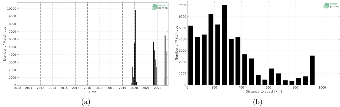
Figure 1: Number of match-ups between Saildrone and SMAP SSS L4 OI v2 - Monthly (IPRC) SSS as a function of time (a) and as function of the distance to coast (b) over the Tropical Atlantic Ocean Pi-MEP region and for the full satellite product period.
