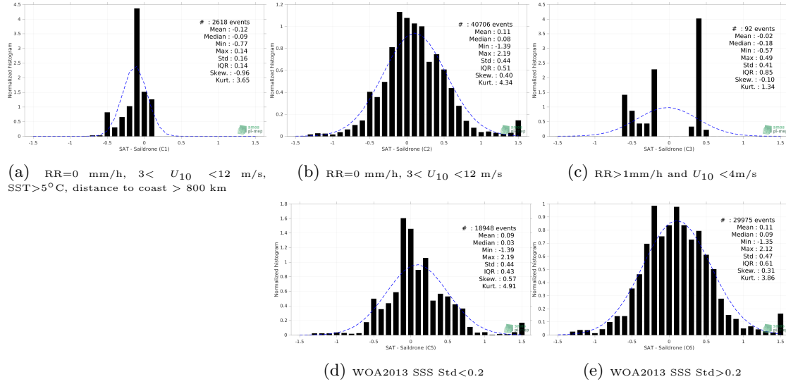
Figure 13: Normalized histogram of \Delta SSS (SMAP SSS L4 OI v2 - Monthly (IPRC) - SSS (Saildrone)) for 5 different subdatasets corresponding to: RR=0 mm/h, 3 < U_{10} < 12 m/s, SST > 5°C, distance to coast > 800 km (a), RR=0 mm/h, 3 < U_{10} < 12 m/s (b), RR > 1mm/h and U_{10} < 4 m/s (c), WOA2013 SSS Std < 0.2 (d), WOA2013 SSS Std > 0.2 (e).
