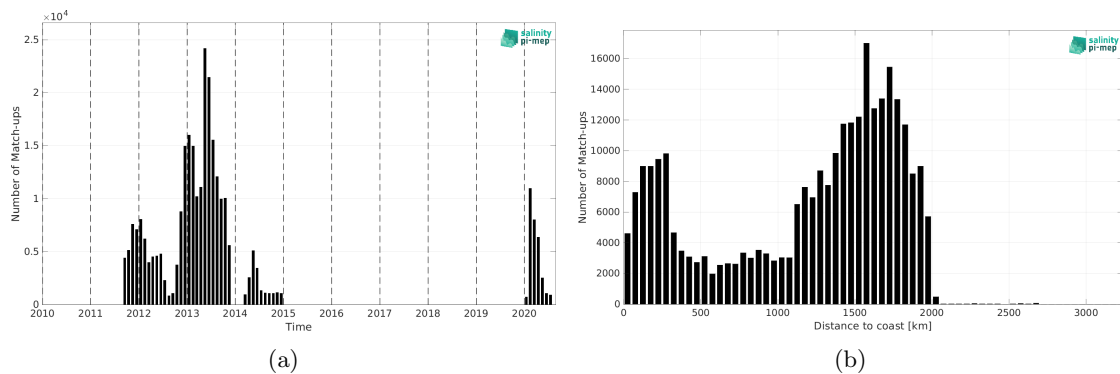
Figure 1: Number of match-ups between Surface drifters and SMAP SSS L4 OI v2 - Monthly (IPRC) SSS as a function of time (a) and as function of the distance to coast (b) over the Tropical Atlantic Ocean Pi-MEP region and for the full satellite product period.
