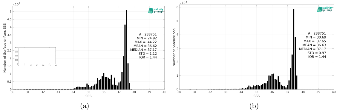
Figure 2: Histograms of SSS from Surface drifters (a) and SMAP SSS L4 OI v2 - Monthly (IPRC) (b) considering all match-up pairs per bins of 0.1 over the Tropical Atlantic Ocean Pi-MEP region and for the full satellite product period.
