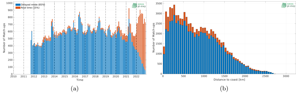
Figure 1: Number of match-ups between Argo and SMAP SSS L4 OI v2 - Monthly (IPRC) SSS as a function of time (a) and as function of the distance to coast (b) over the Tropical Atlantic Ocean Pi-MEP region and for the full satellite product period.
