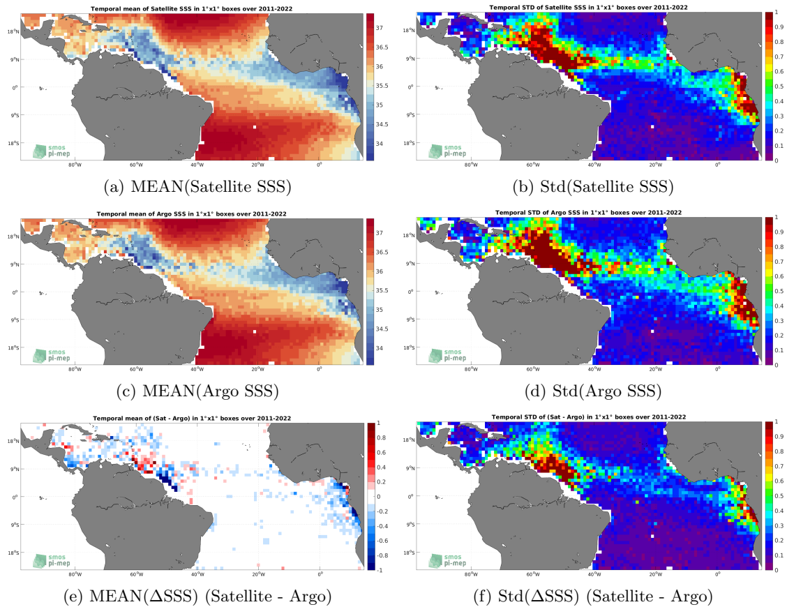
Figure 6: Temporal mean (left) and Std (right) of SSS from SMAP SSS L4 OI v2 - Monthly (IPRC) (top), Argo (middle), and of \Delta SSS (Satellite - Argo). Only match-up pairs are used to generate these maps.
