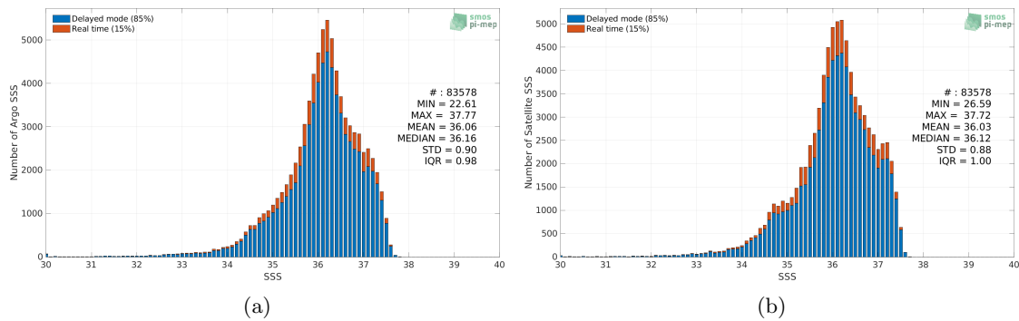
Figure 2: Histograms of SSS from Argo (a) and SMAP SSS L4 OI v2 - Monthly (IPRC) (b) considering all match-up pairs per bins of 0.1 over the Tropical Atlantic Ocean Pi-MEP region and for the full satellite product period.
