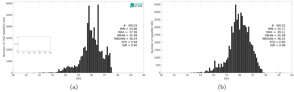
Figure 3: Histograms of SSS from TSG (SAMOS) (a) and SMAP SSS L3 v6 - 8-Day running (RSS) (b) considering all match-up pairs per bins of 0.1 over the Tropical Atlantic Ocean Pi-MEP region and for the full satellite product period.
