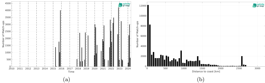
Figure 2: Number of match-ups between TSG (SAMOS) and SMAP SSS L3 v6 - 8-Day running (RSS) SSS as a function of time (a) and as function of the distance to coast (b) over the Tropical Atlantic Ocean Pi-MEP region and for the full satellite product period.
