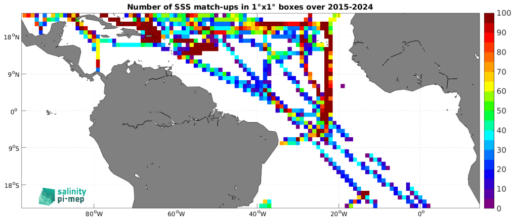
Figure 5: Number of SSS match-ups between TSG (SAMOS) SSS and the SMAP SSS L3 v6 - 8-Day running (RSS) SSS product for the Tropical Atlantic Ocean Pi-MEP region over 1^\circ \times 1^\circ boxes and for the full satellite product period.
