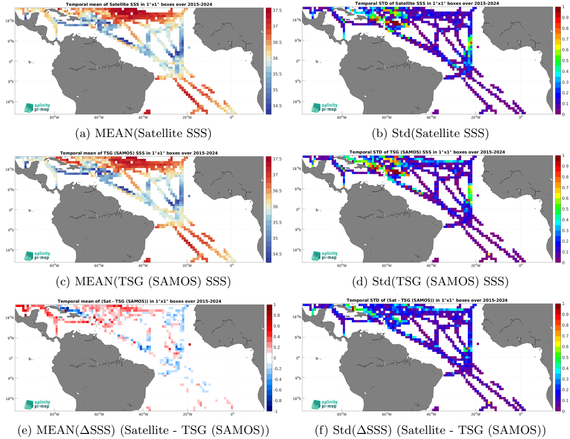
Figure 7: Temporal mean (left) and Std (right) of SSS from SMAP SSS L3 v6 - 8-Day running (RSS) (top), TSG (SAMOS) (middle), and of \Delta\text{SSS} (Satellite - TSG (SAMOS)). Only match-up pairs are used to generate these maps.
