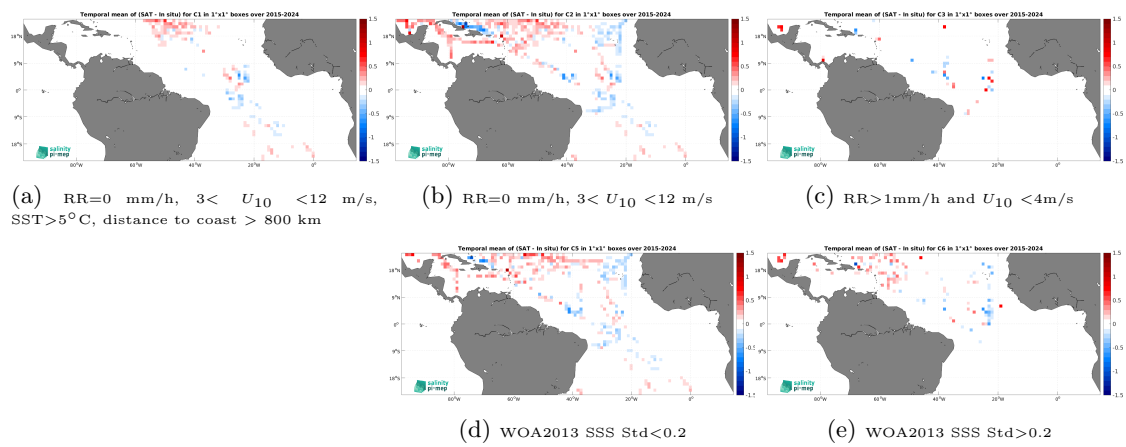
Figure 14: Temporal mean gridded over spatial boxes of size 1^\circ \times 1^\circ of \Delta\text{SSS} (SMAP SSS L3 v6 - 8-Day running (RSS) - TSG (SAMOS)) for 5 different subdatasets corresponding to:RR=0 mm/h, 3 < U_{10} < 12 m/s, SST >5^\circ\text{C} , distance to coast > 800 km (a), RR=0 mm/h, 3 < U_{10} < 12 m/s (b), RR >1 mm/h and U_{10} < 4 m/s (c), WOA2013 SSS Std <0.2 (d), WOA2013 SSS Std >0.2 (e).
