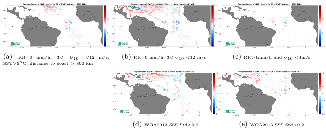
Figure 14: Temporal mean gridded over spatial boxes of size 1^\circ \times 1^\circ of \Delta\text{SSS} (SMAP SSS L3 v6 - 8-Day running (RSS) - TSG (SAMOS)) for 5 different subdatasets corresponding to:RR=0 mm/h, 3 < U_{10} < 12 m/s, SST >5^\circ\text{C} , distance to coast > 800 km (a), RR=0 mm/h, 3 < U_{10} < 12 m/s (b), RR >1 mm/h and U_{10} < 4 m/s (c), WOA2013 SSS Std <0.2 (d), WOA2013 SSS Std >0.2 (e).
