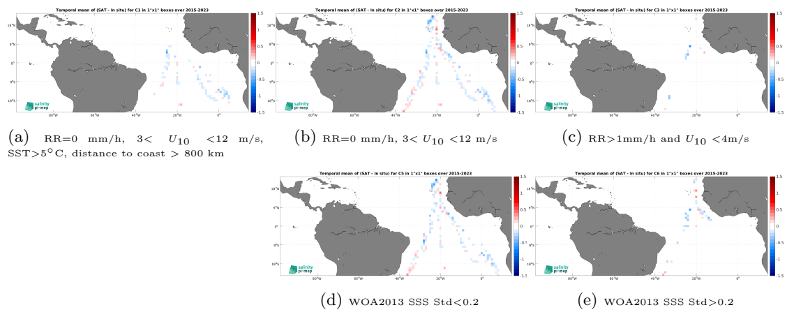
Figure 14: Temporal mean gridded over spatial boxes of size 1^\circ \times 1^\circ of \Delta\text{SSS} (SMAP SSS L3 v6 - 8-Day running (RSS) - TSG (Polarstern)) for 5 different subdatasets corresponding to:RR=0 mm/h, 3 < U_{10} < 12 m/s, SST >5^\circ\text{C} , distance to coast > 800 km (a), RR=0 mm/h, 3 < U_{10} < 12 m/s (b), RR >1 mm/h and U_{10} < 4 m/s (c), WOA2013 SSS Std <0.2 (d), WOA2013 SSS Std >0.2 (e).
