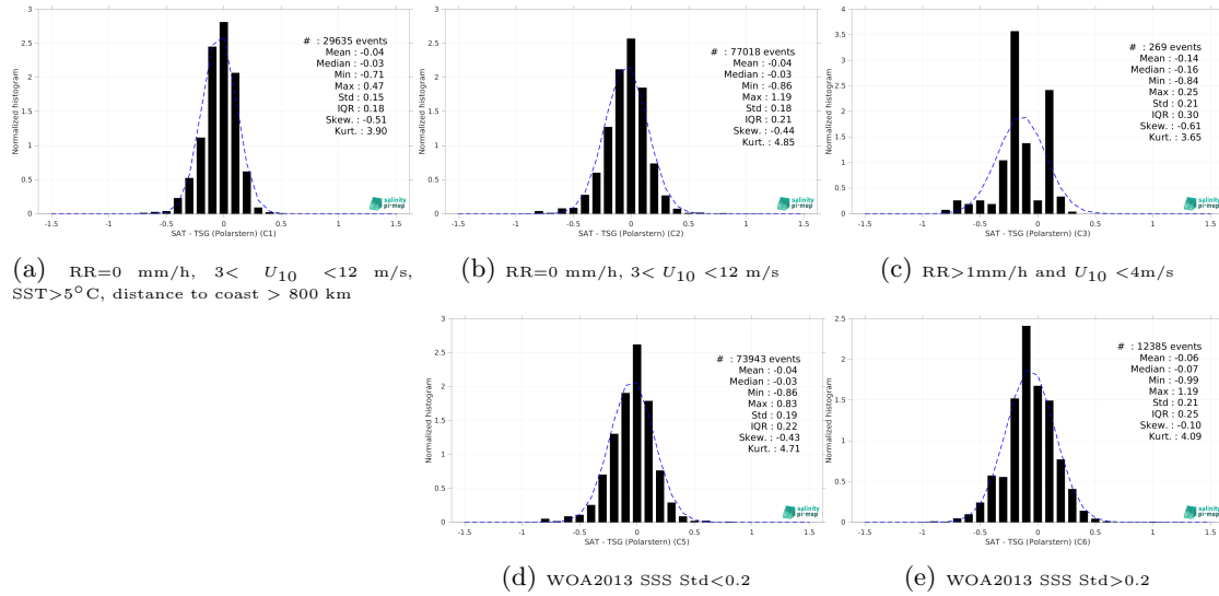
Figure 15: Normalized histogram of \Delta SSS (SMAP SSS L3 v6 - 8-Day running (RSS) - TSG (Polarstern)) for 5 different subdatasets corresponding to: RR=0 mm/h, 3 < U_{10} < 12 m/s, SST>5°C, distance to coast > 800 km (a), RR=0 mm/h, 3 < U_{10} < 12 m/s (b), RR>1mm/h and U_{10} < 4 m/s (c), WOA2013 SSS Std<0.2 (d), WOA2013 SSS Std>0.2 (e).
