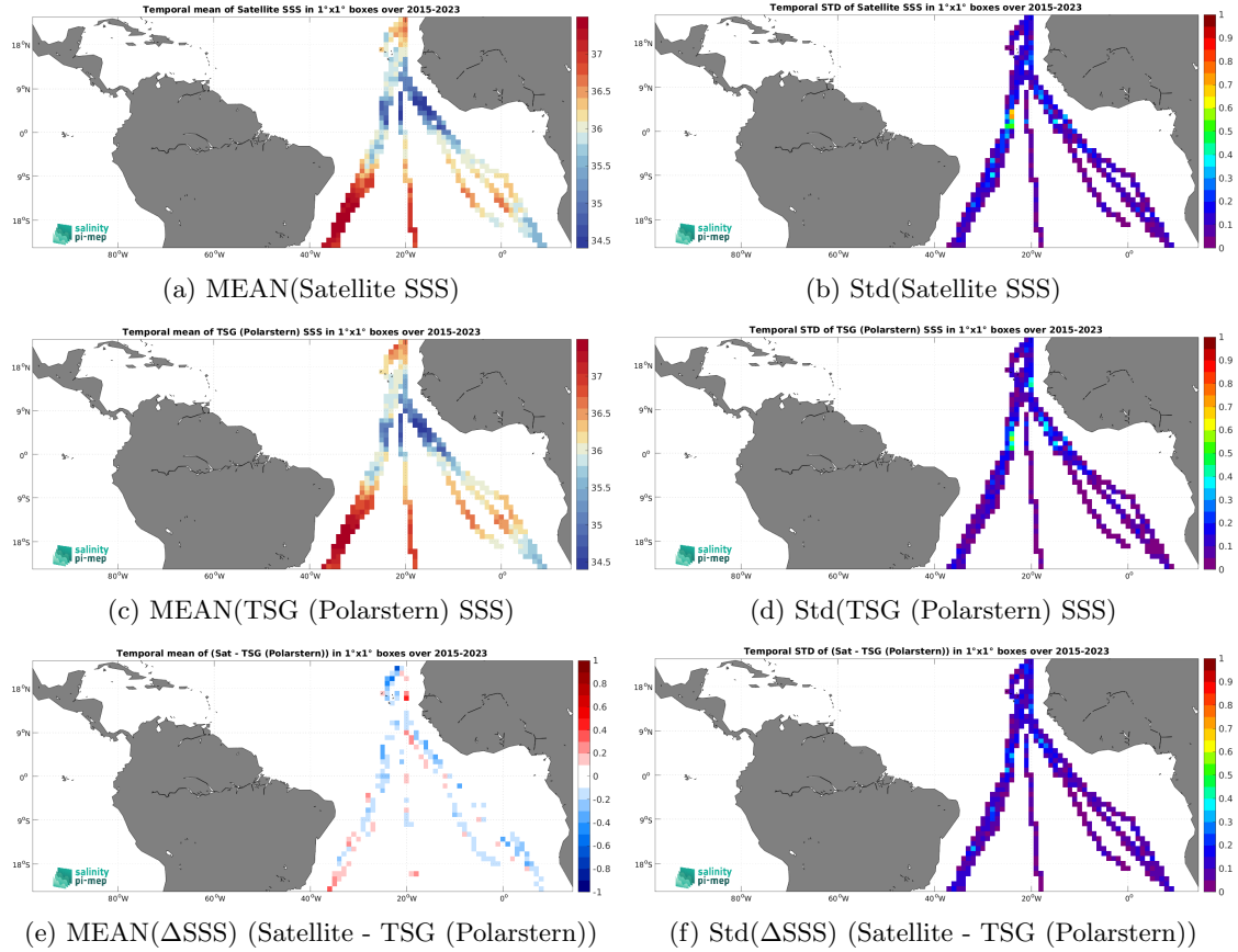
Figure 7: Temporal mean (left) and Std (right) of SSS from SMAP SSS L3 v6 - 8-Day running (RSS) (top), TSG (Polarstern) (middle), and of \Delta\text{SSS} (Satellite - TSG (Polarstern)). Only match-up pairs are used to generate these maps.
