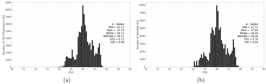
Figure 3: Histograms of SSS from TSG (Polarstern) (a) and SMAP SSS L3 v6 - 8-Day running (RSS) (b) considering all match-up pairs per bins of 0.1 over the Tropical Atlantic Ocean Pi-MEP region and for the full satellite product period.
