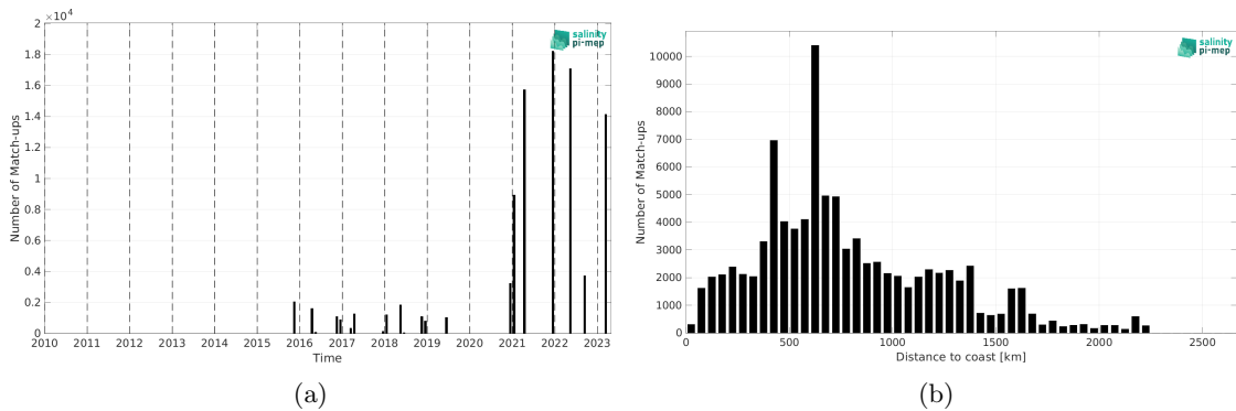
Figure 2: Number of match-ups between TSG (Polarstern) and SMAP SSS L3 v6 - 8-Day running (RSS) SSS as a function of time (a) and as function of the distance to coast (b) over the Tropical Atlantic Ocean Pi-MEP region and for the full satellite product period.
