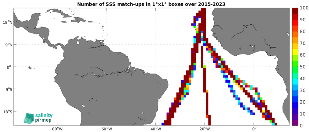
Figure 5: Number of SSS match-ups between TSG (Polarstern) SSS and the SMAP SSS L3 v6 - 8-Day running (RSS) SSS product for the Tropical Atlantic Ocean Pi-MEP region over 1^\circ \times 1^\circ boxes and for the full satellite product period.
