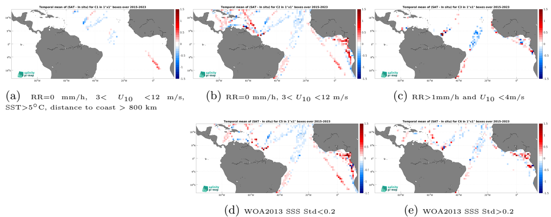
Figure 14: Temporal mean gridded over spatial boxes of size 1^\circ \times 1^\circ of \Delta\text{SSS} (SMAP SSS L3 v6 - 8-Day running (RSS) - TSG (LEGOS-DM)) for 5 different subdatasets corresponding to:RR=0 mm/h, 3 < U_{10} < 12 m/s, SST >5^\circ\text{C} , distance to coast > 800 km (a), RR=0 mm/h, 3 < U_{10} < 12 m/s (b), RR >1 mm/h and U_{10} < 4 m/s (c), WOA2013 SSS Std <0.2 (d), WOA2013 SSS Std >0.2 (e).
