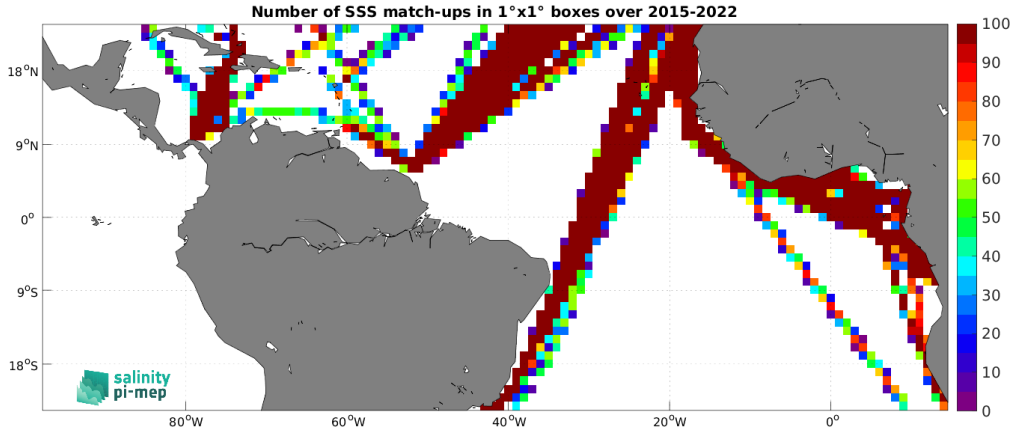
Figure 5: Number of SSS match-ups between TSG (LEGOS-DM) SSS and the SMAP SSS L3 v6 - 8-Day running (RSS) SSS product for the Tropical Atlantic Ocean Pi-MEP region over 1^\circ \times 1^\circ boxes and for the full satellite product period.
