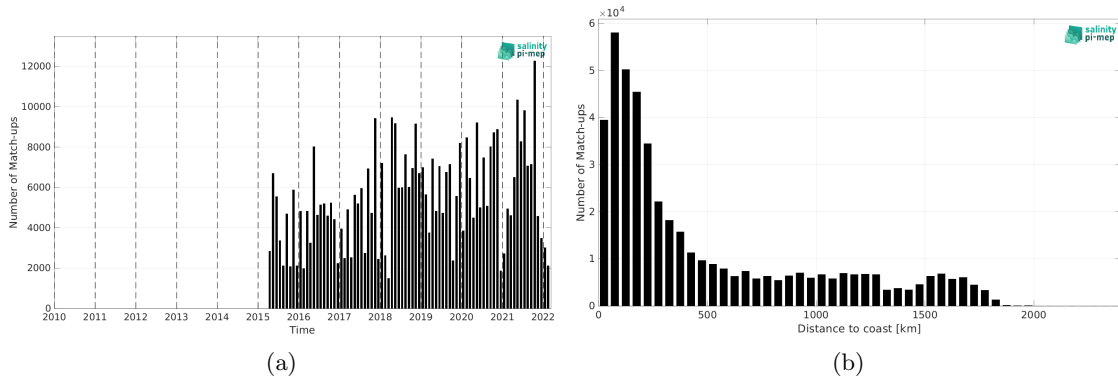
Figure 2: Number of match-ups between TSG (LEGOS-DM) and SMAP SSS L3 v6 - 8-Day running (RSS) SSS as a function of time (a) and as function of the distance to coast (b) over the Tropical Atlantic Ocean Pi-MEP region and for the full satellite product period.
