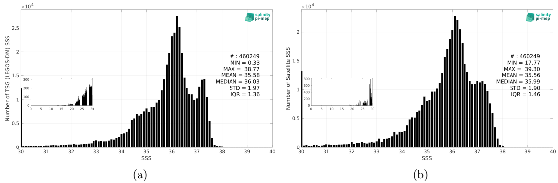
Figure 3: Histograms of SSS from TSG (LEGOS-DM) (a) and SMAP SSS L3 v6 - 8-Day running (RSS) (b) considering all match-up pairs per bins of 0.1 over the Tropical Atlantic Ocean Pi-MEP region and for the full satellite product period.
