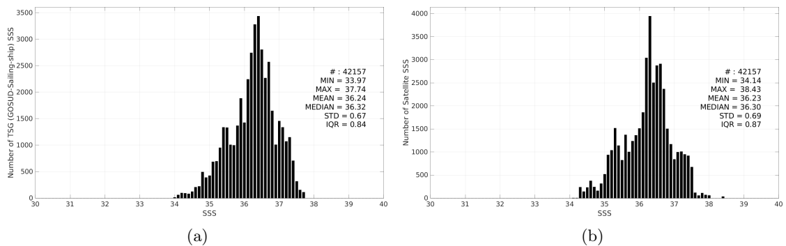
Figure 3: Histograms of SSS from TSG (GOSUD-Sailing-ship) (a) and SMAP SSS L3 v6 - 8-Day running (RSS) (b) considering all match-up pairs per bins of 0.1 over the Tropical Atlantic Ocean Pi-MEP region and for the full satellite product period.
