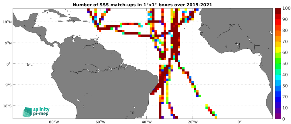
Figure 5: Number of SSS match-ups between TSG (GOSUD-Sailing-ship) SSS and the SMAP SSS L3 v6 - 8-Day running (RSS) SSS product for the Tropical Atlantic Ocean Pi-MEP region over 1^\circ \times 1^\circ boxes and for the full satellite product period.
