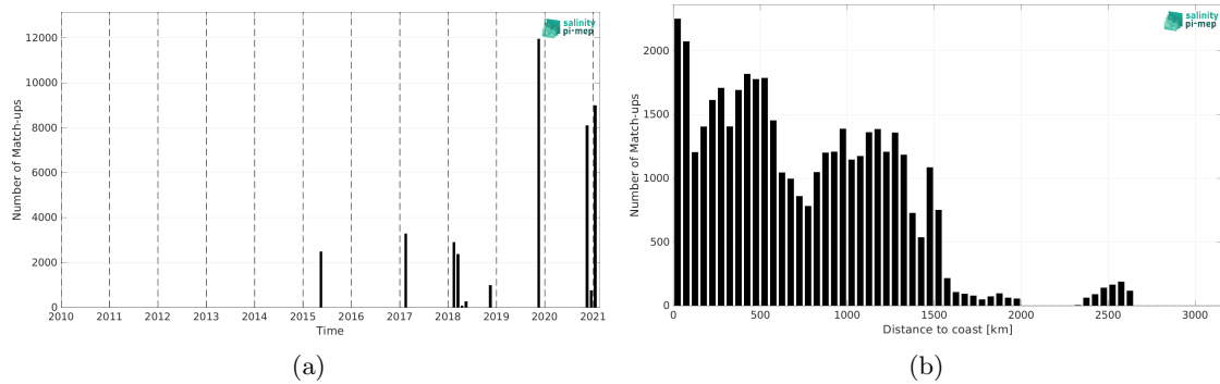
Figure 2: Number of match-ups between TSG (GOSUD-Sailing-ship) and SMAP SSS L3 v6 - 8-Day running (RSS) SSS as a function of time (a) and as function of the distance to coast (b) over the Tropical Atlantic Ocean Pi-MEP region and for the full satellite product period.
