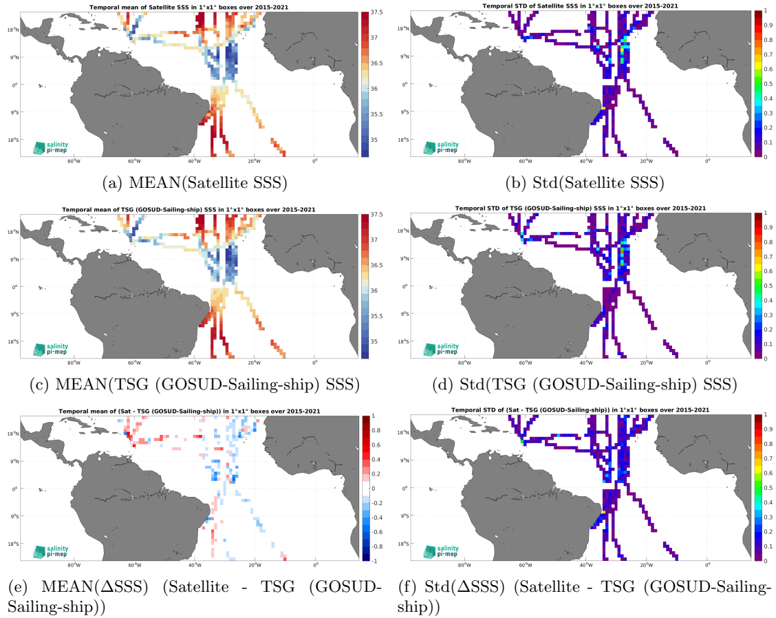
Figure 7: Temporal mean (left) and Std (right) of SSS from SMAP SSS L3 v6 - 8-Day running (RSS), TSG (GOSUD-Sailing-ship) (middle), and of \Delta SSS (Satellite - TSG (GOSUD-Sailing-ship)). Only match-up pairs are used to generate these maps.
